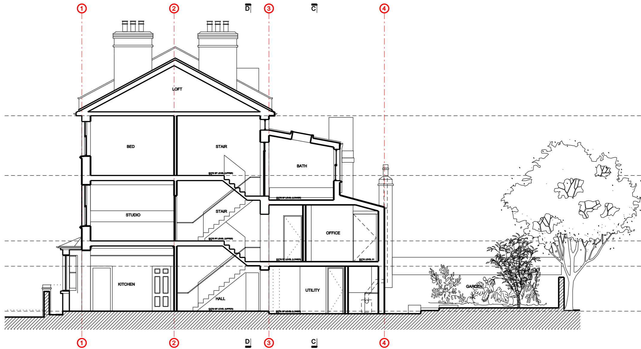
01 EXISTING SECTION BB SCALE 1:100 AT A3
