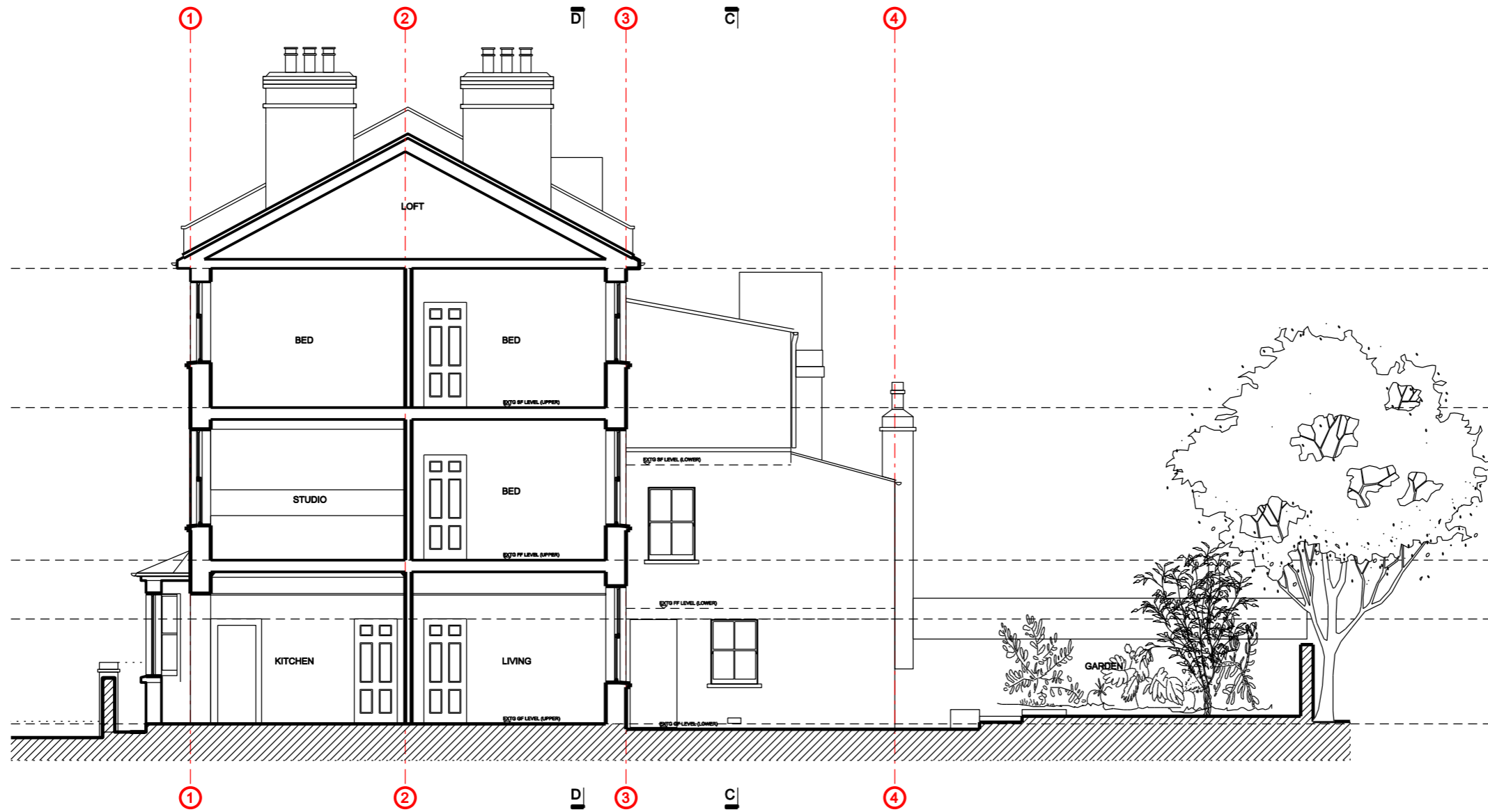
01 EXISTING SECTION AA SCALE 1:100 AT A3
