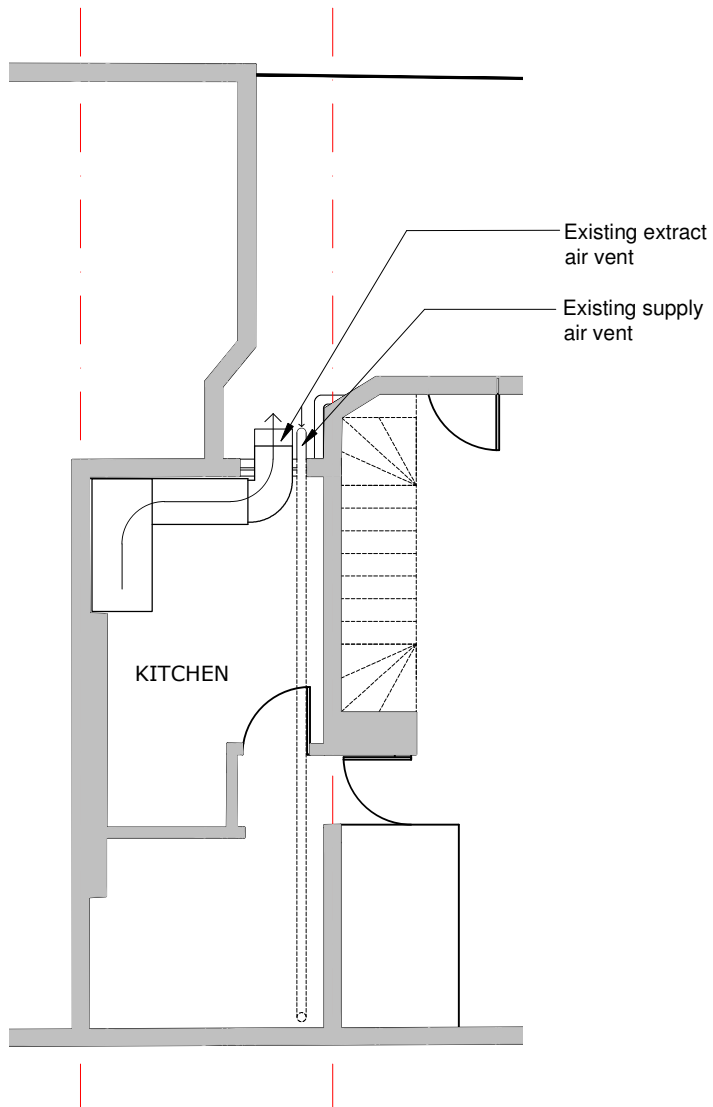
BASEMENT FLOOR - EXISTING
