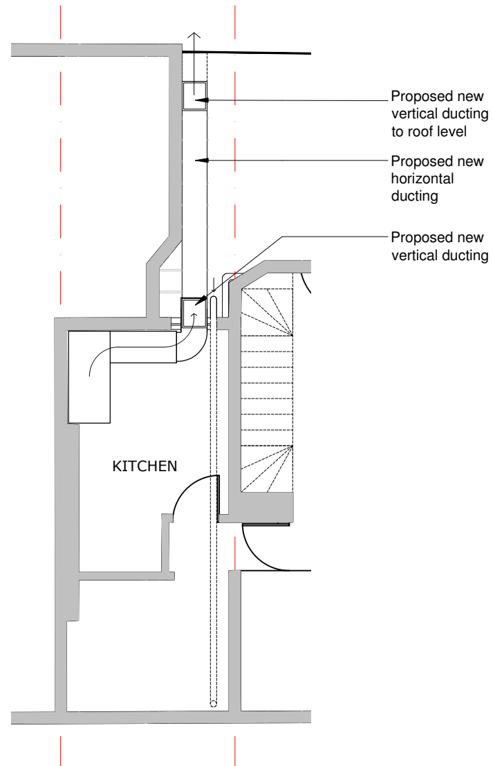
BASEMENT FLOOR - PROPOSED
