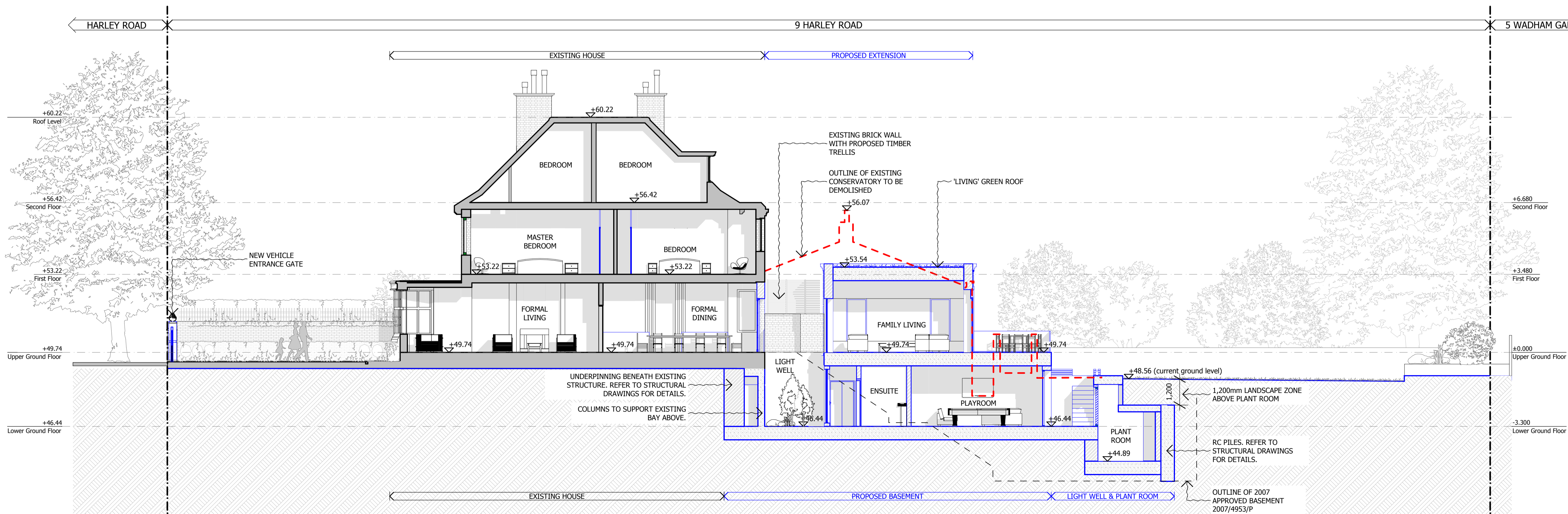
2 SECTION AA - PROPOSED
