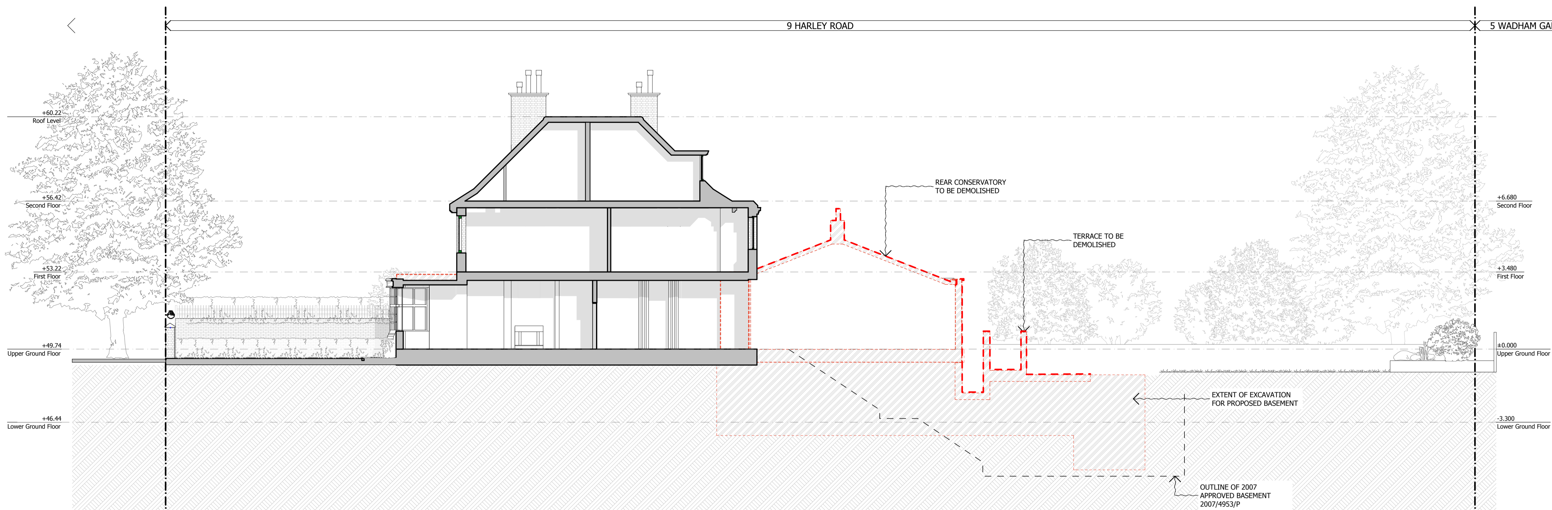
1 SECTION AA - EXISTING/DEMOLITION
