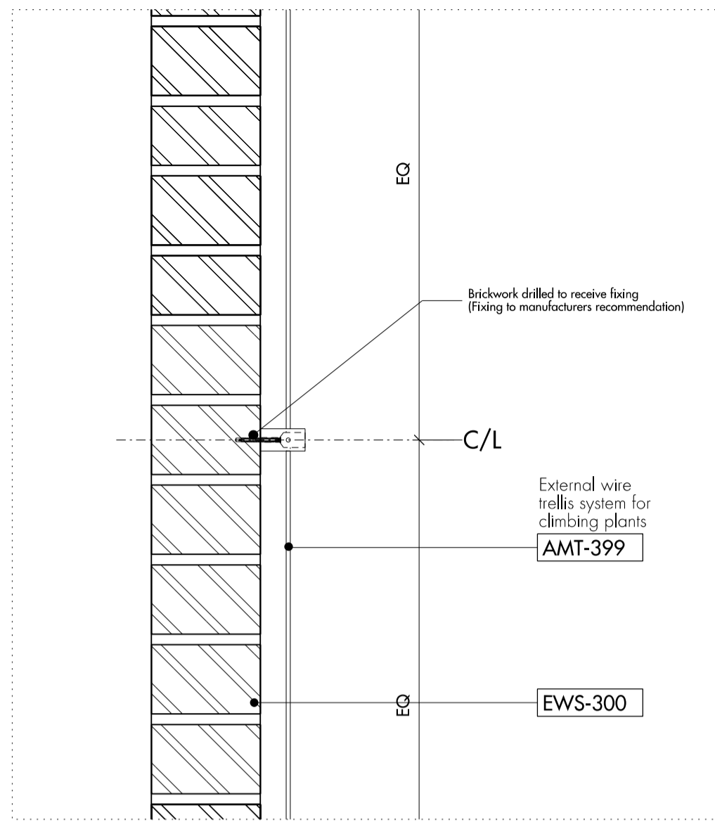
02 GREEN WALL SYSTEM DETAIL ELEVATION 01 SCALE 1:50
