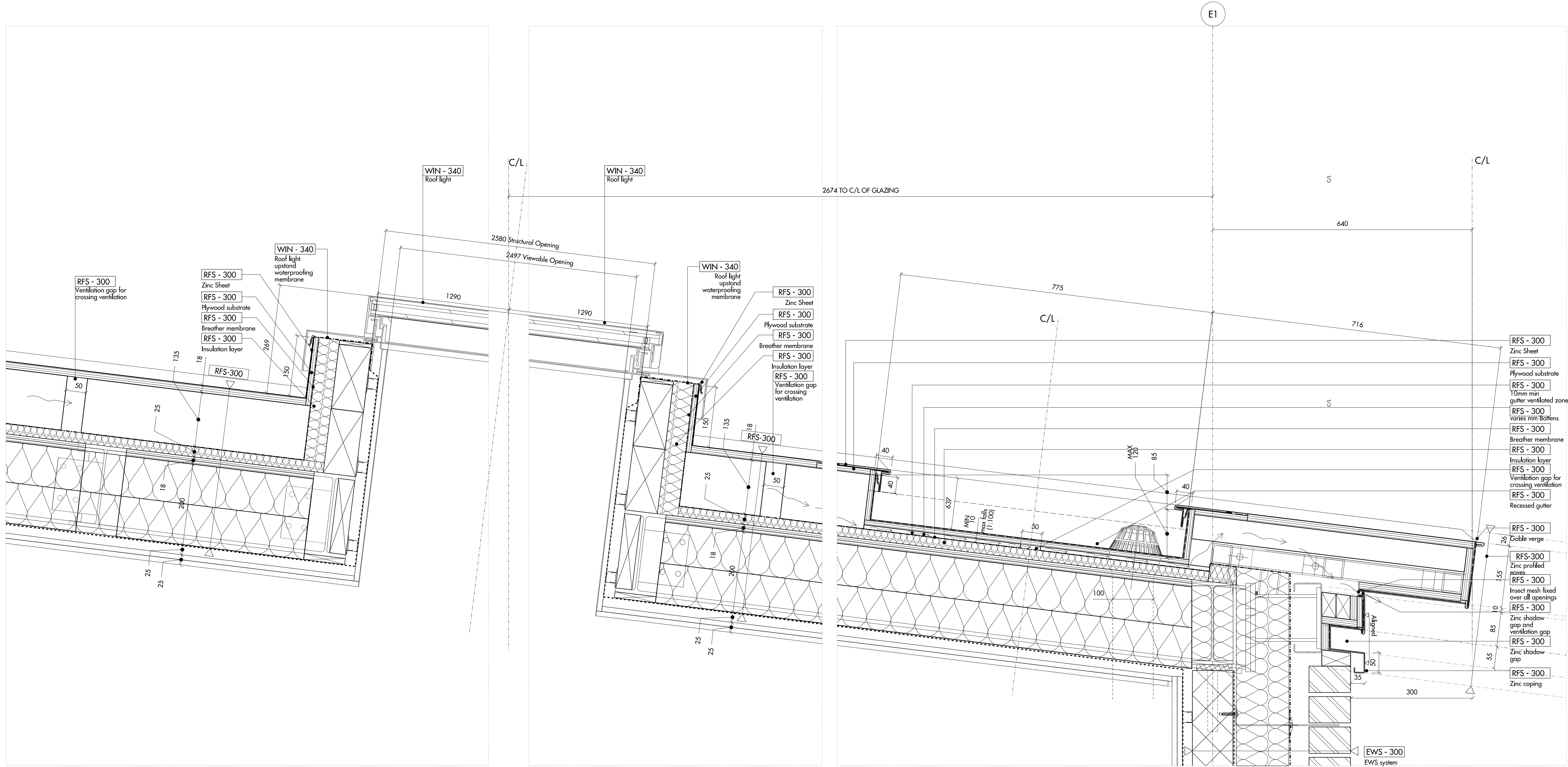
01 ROOF LIGHT DETAIL
