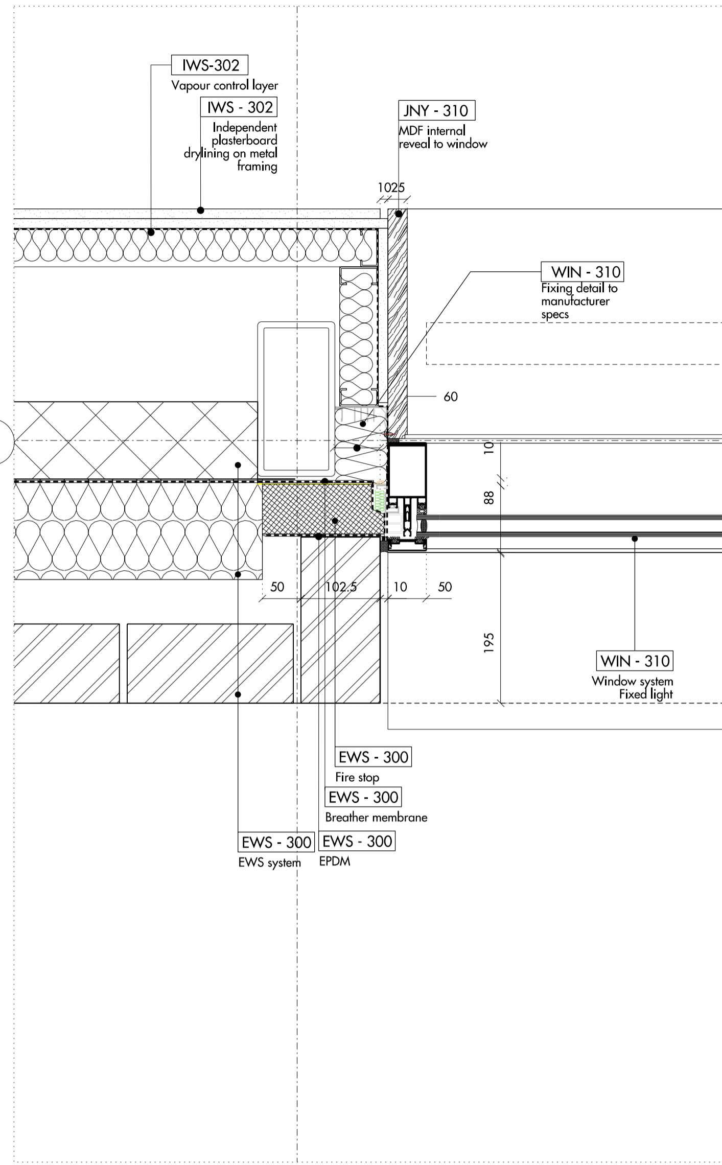
02 WIN - 310_PLAN DETAILS_LEVEL -02
