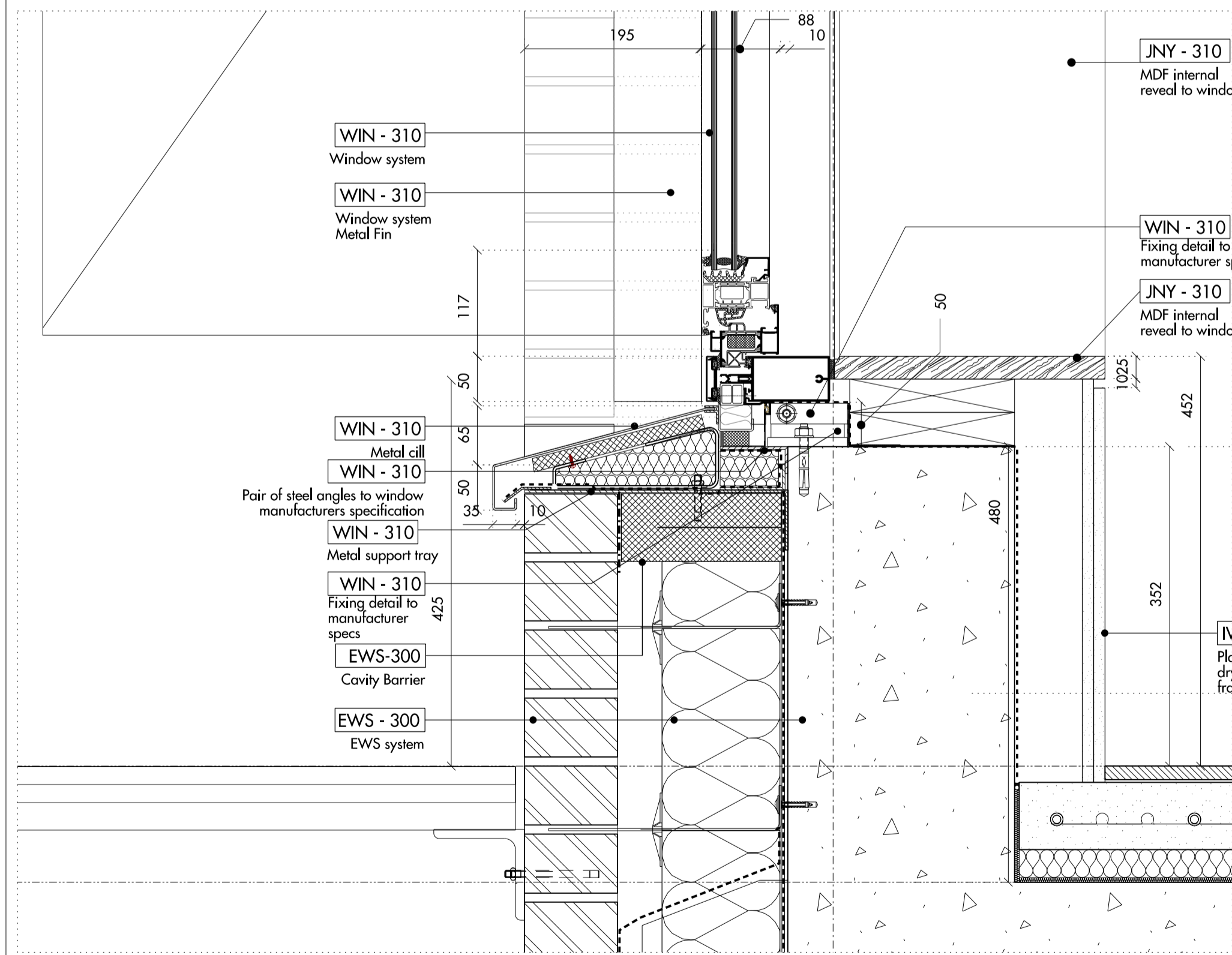
01 WIN - 310_SECTION DETAILS
