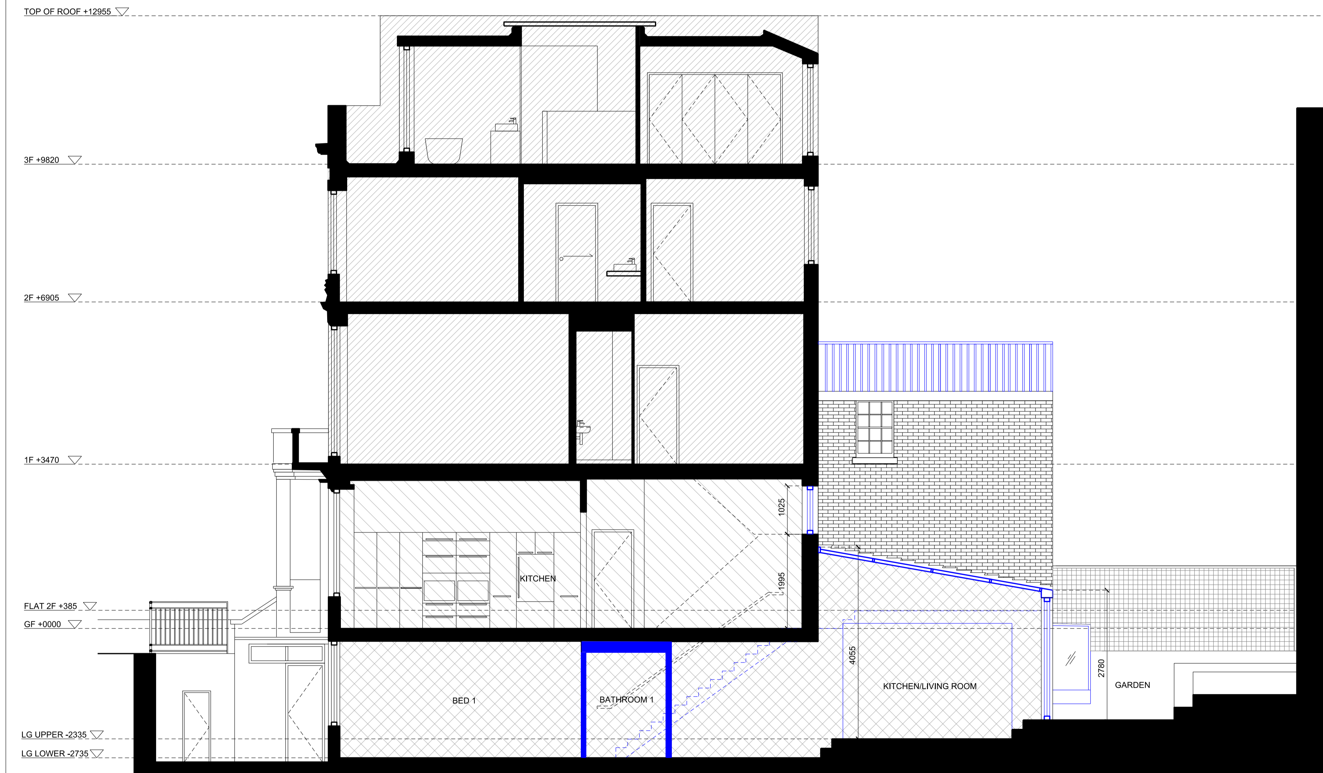
01 - SECTION B-B
