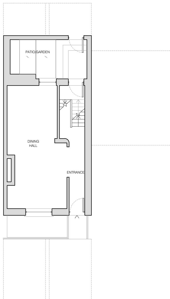
01 EXISTING GROUND FLOOR PLAN scale 1:100
