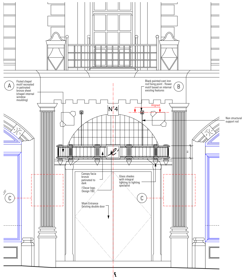
1 Elevation 1:25@A1, 1:50@A3
