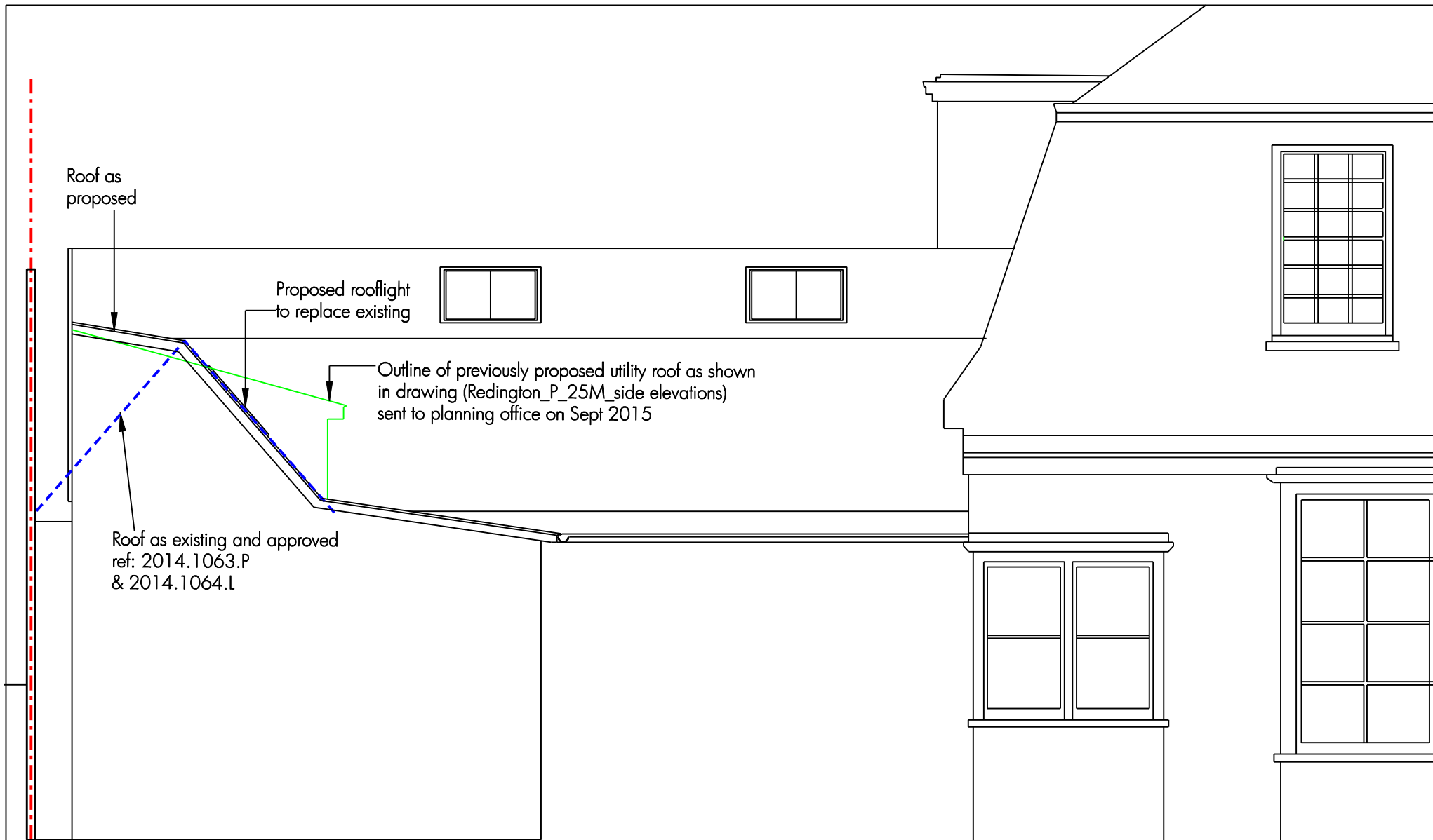
PROPOSED NORTH WEST ELEVATION SK31L - Kitchen side elevation Scale 1:50 @ A4
