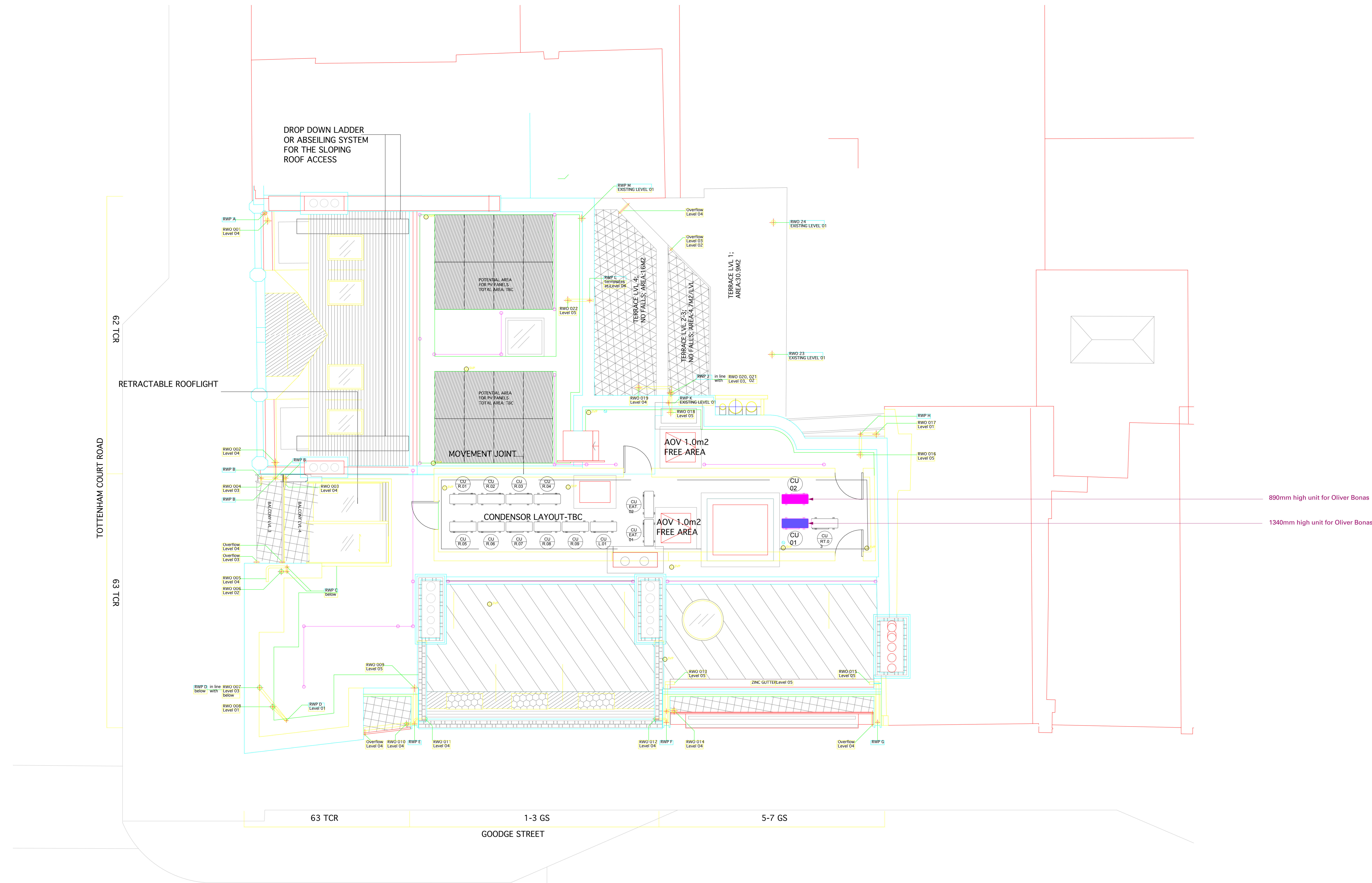
Roof Plan Scale 1:50
