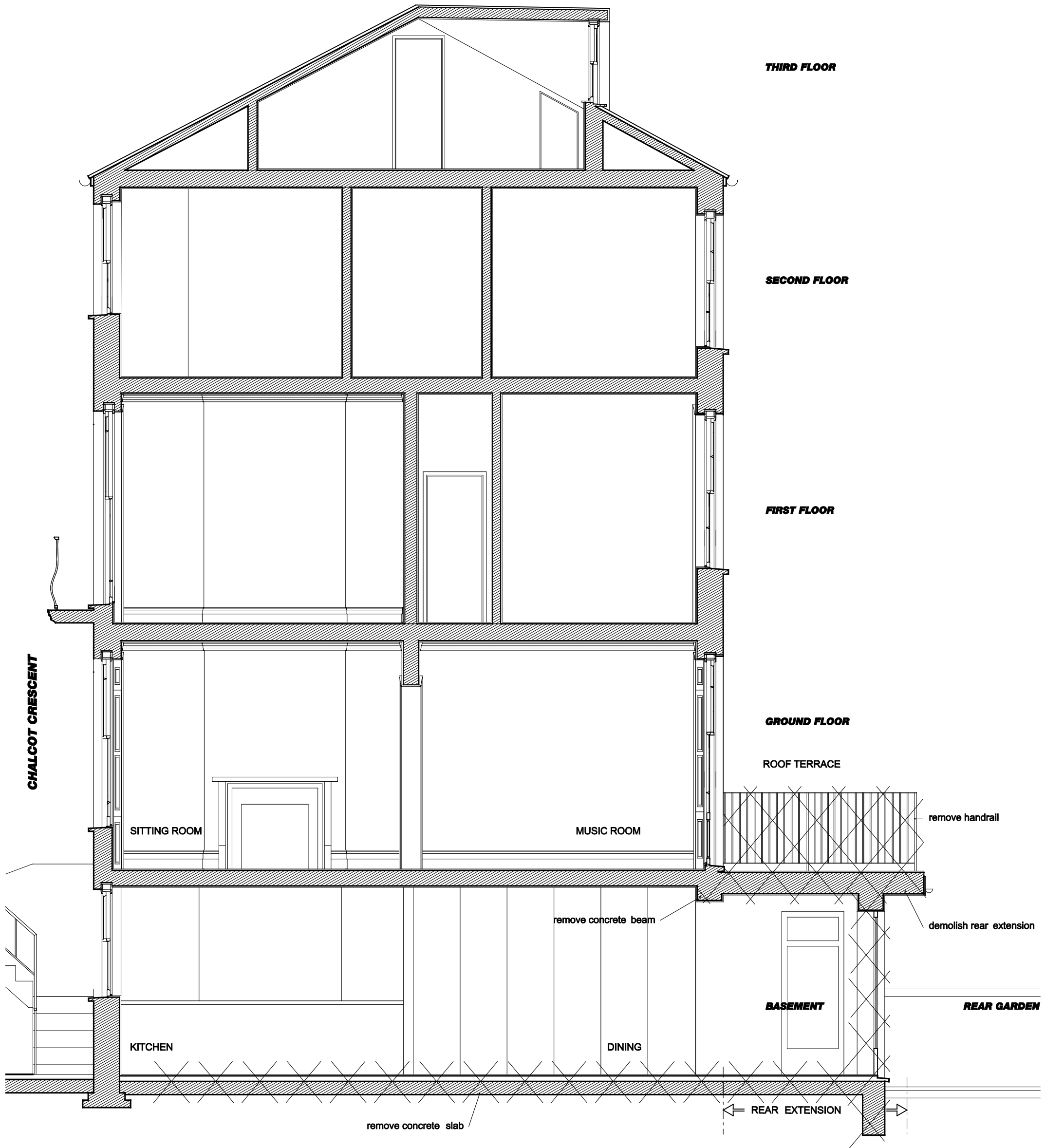
CROSS SECTION
