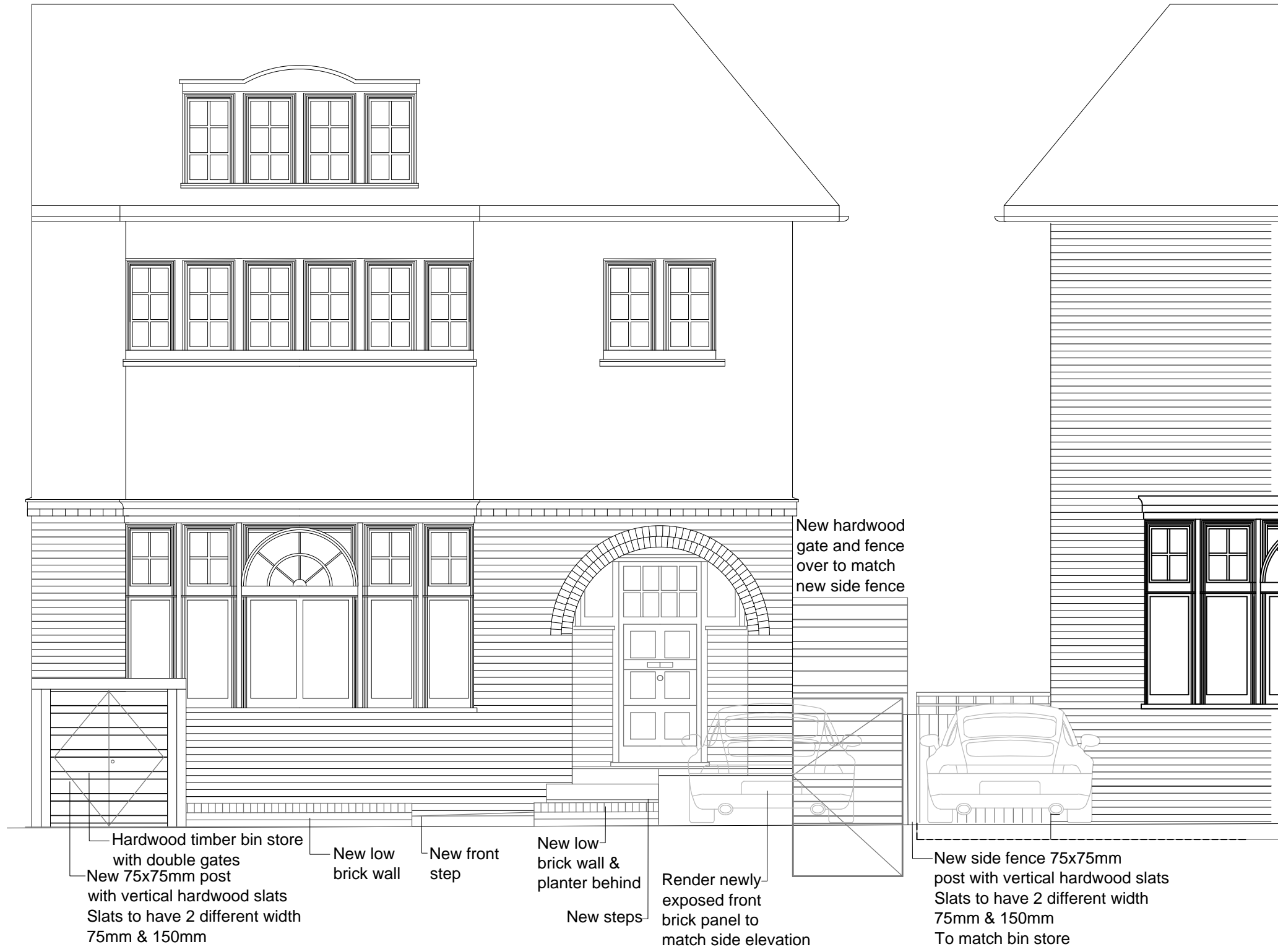
Elevation 1:50 scale
