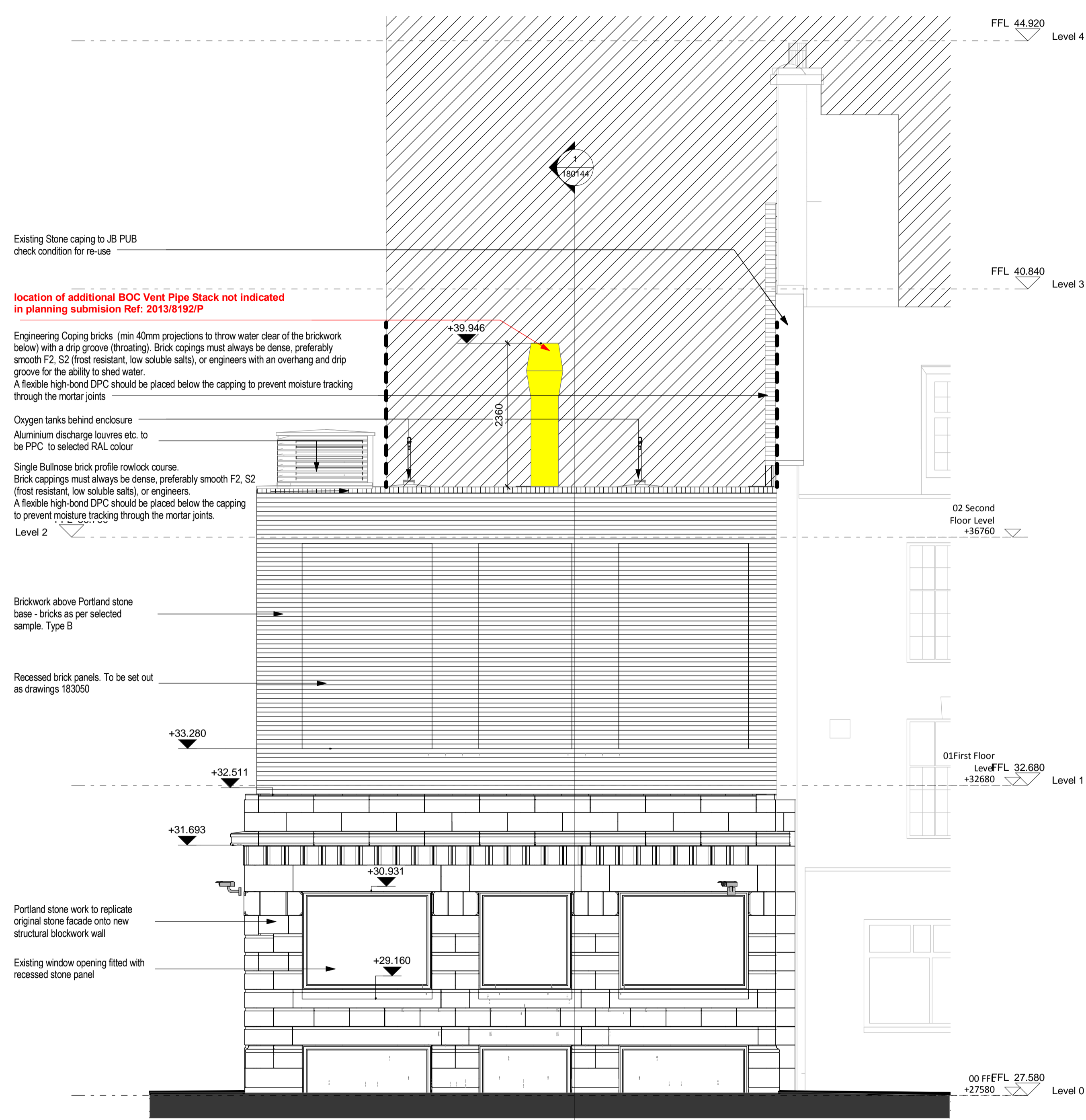
1 180143 VIE - Elevation University Street 1-50 1 : 50
