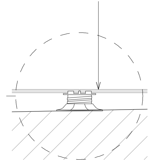
RAISED FLOOR DETAIL, 1:10
