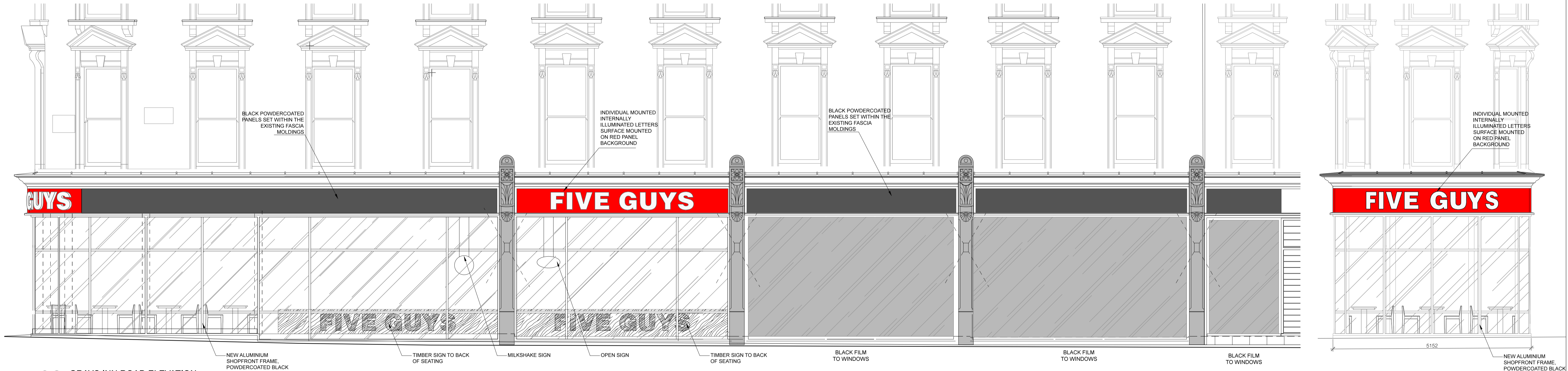
02 GRAYS INN ROAD ELEVATION SCALE 1:50 @ A1
