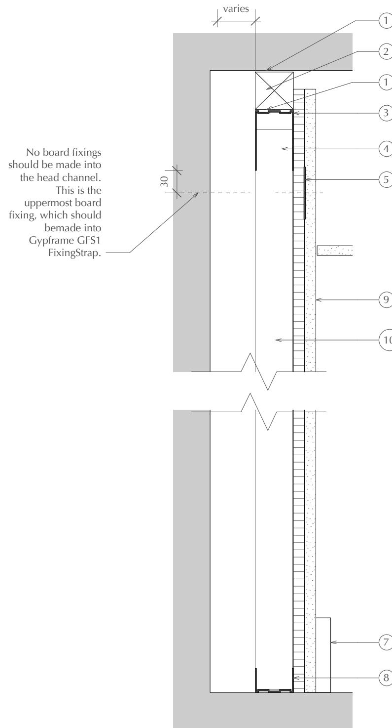
Type H - Plasterboard Boxing out with Ply backing
