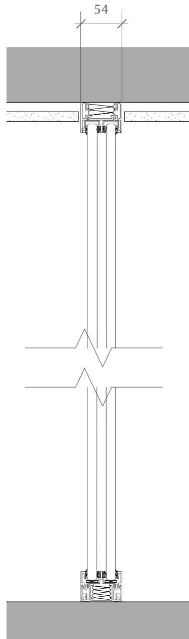
Type E - Glazed partition system with glass door (1:5)
