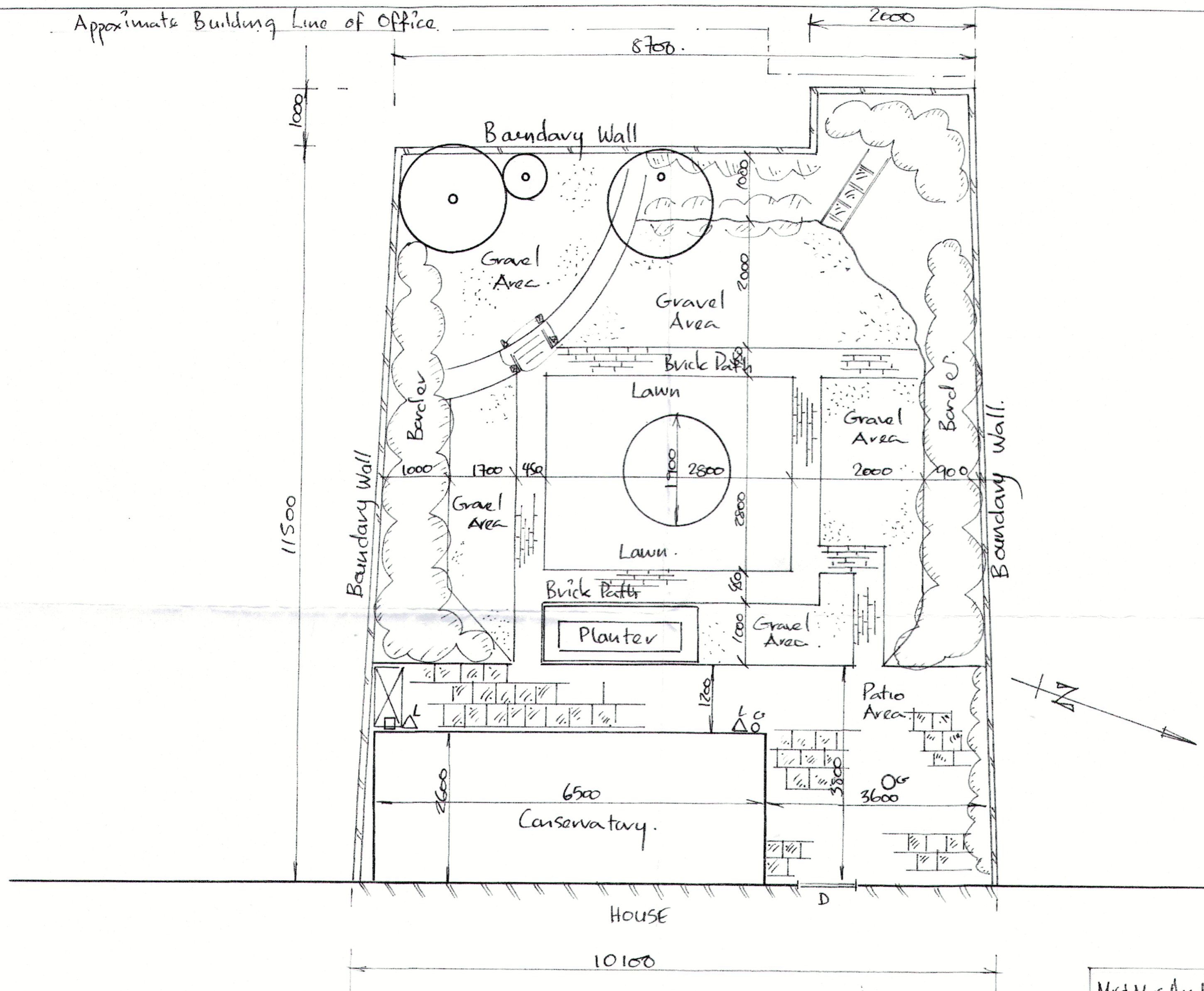
Existing Plan Layout Rear Garden Scale 1:50.
