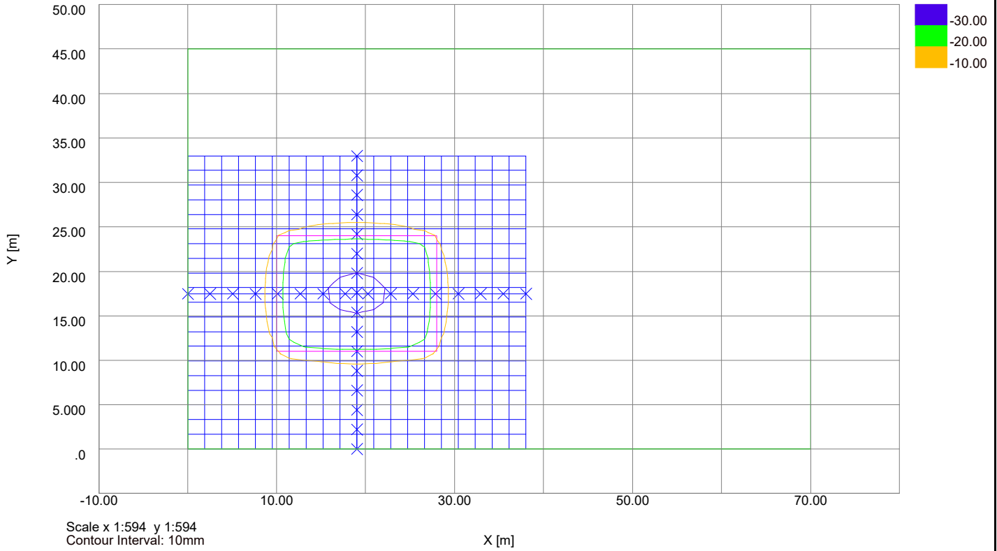
Settlement Contours : Grid 1 at 48.5000m
