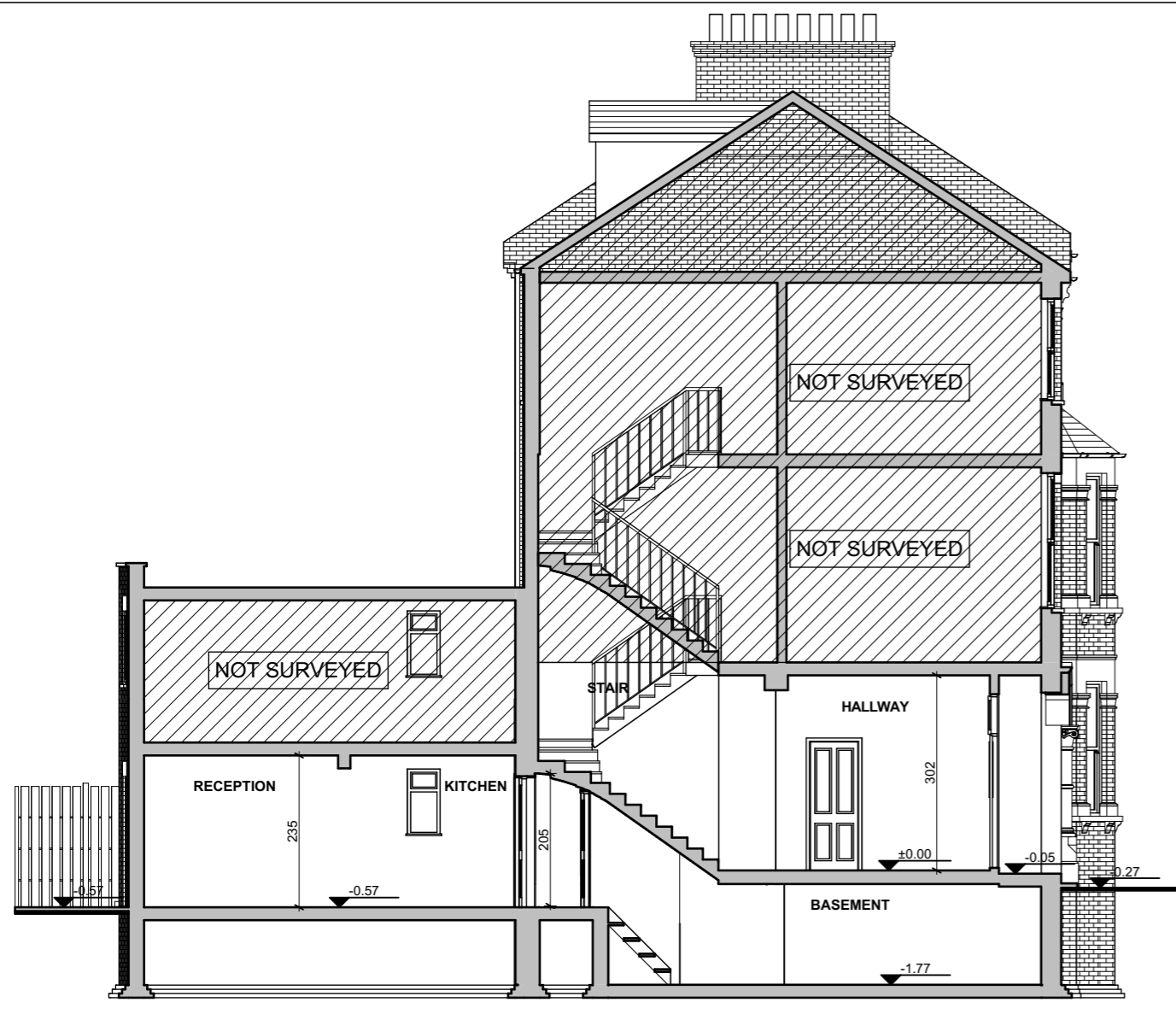
SECTION AA - EXISTING
