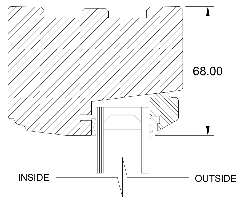
SECTION I scale 1:1
