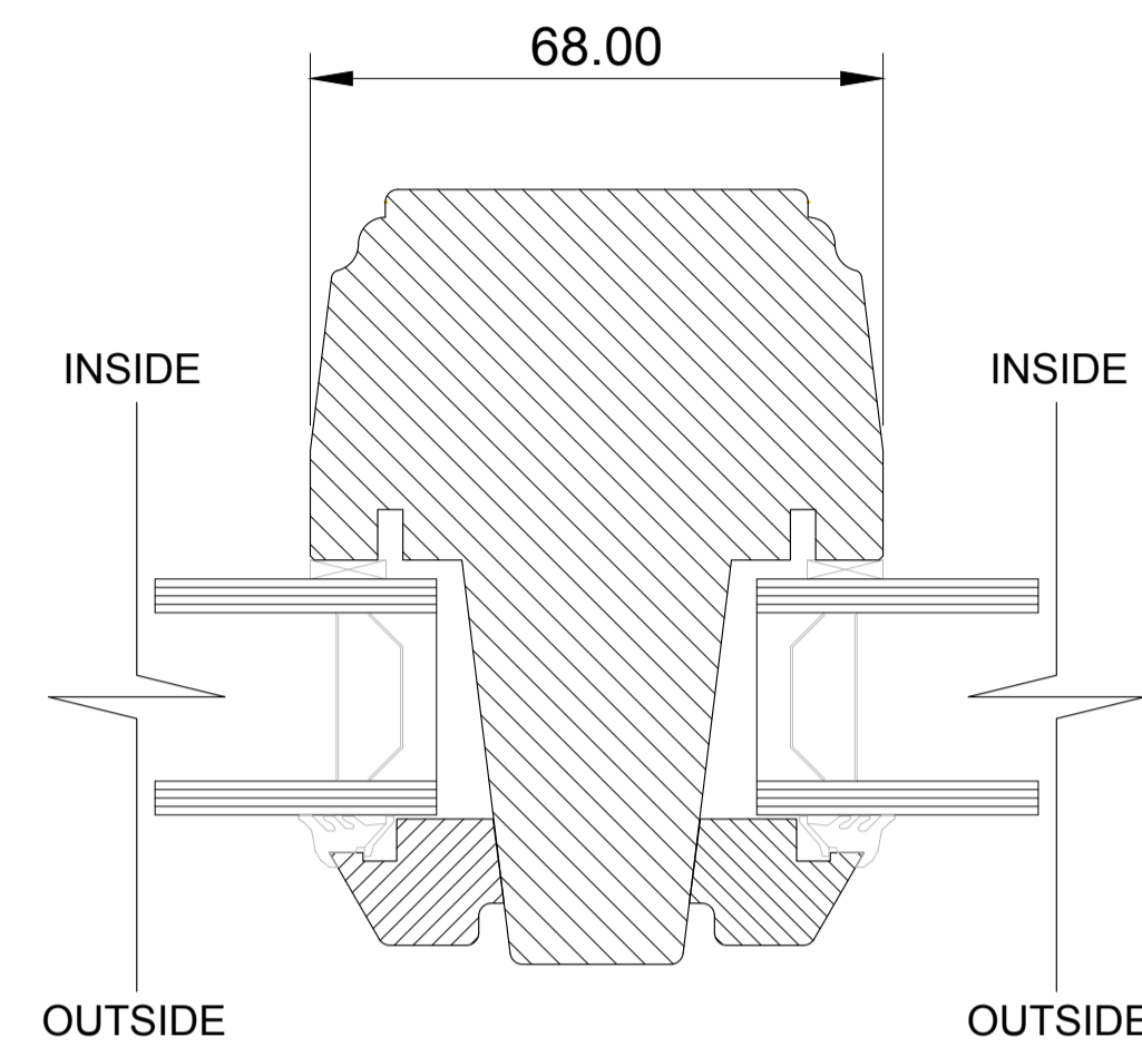
SECTION J scale 1:1
