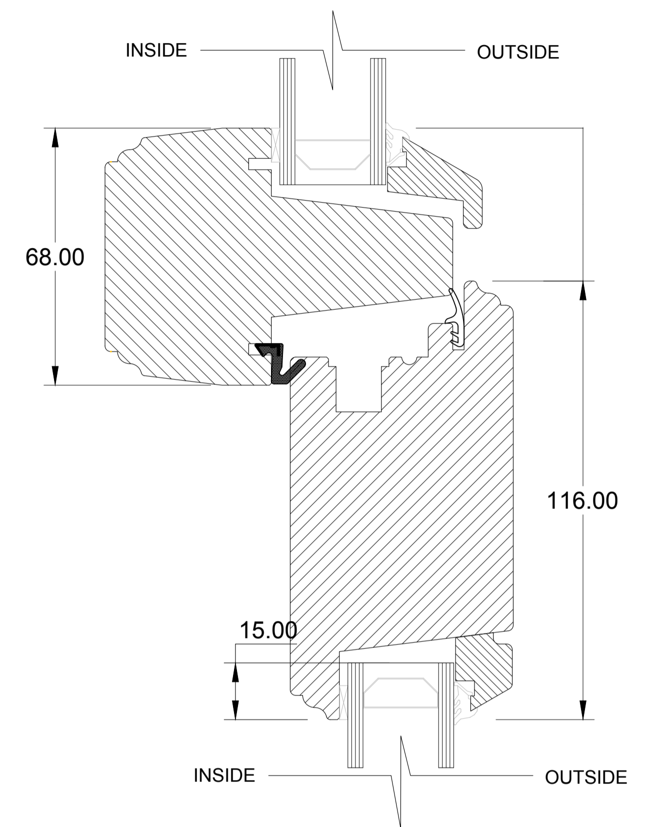
SECTION K scale 1:1
