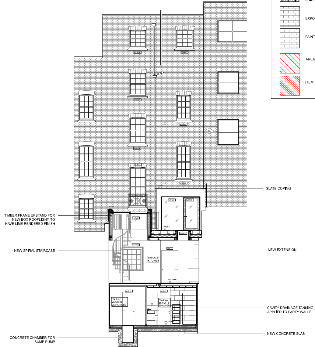
PROPOSED SECTION EE
