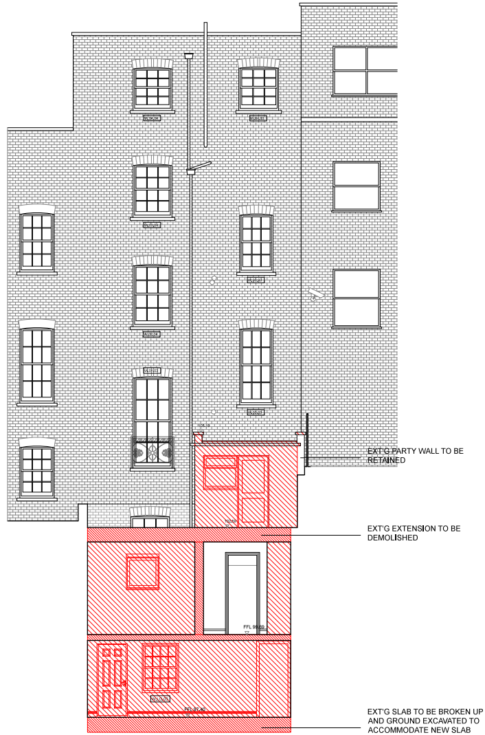
EXISTING SECTION EE
