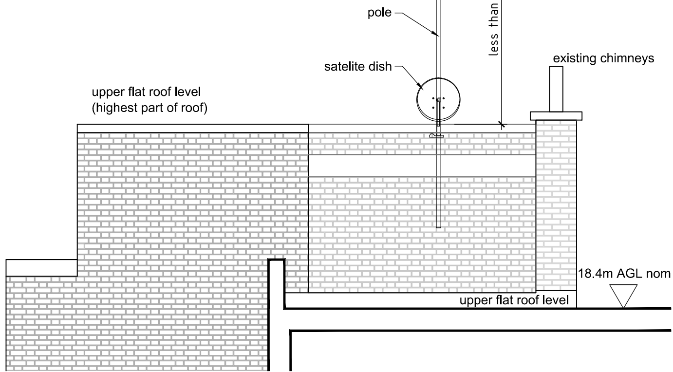
Elevation AA of Proposed Satellite Dish + Aerial Scale 1:50
