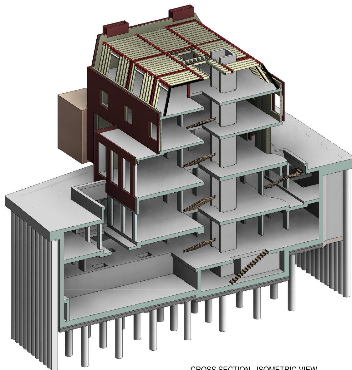
CROSS SECTION - ISOMETRIC VIEW
