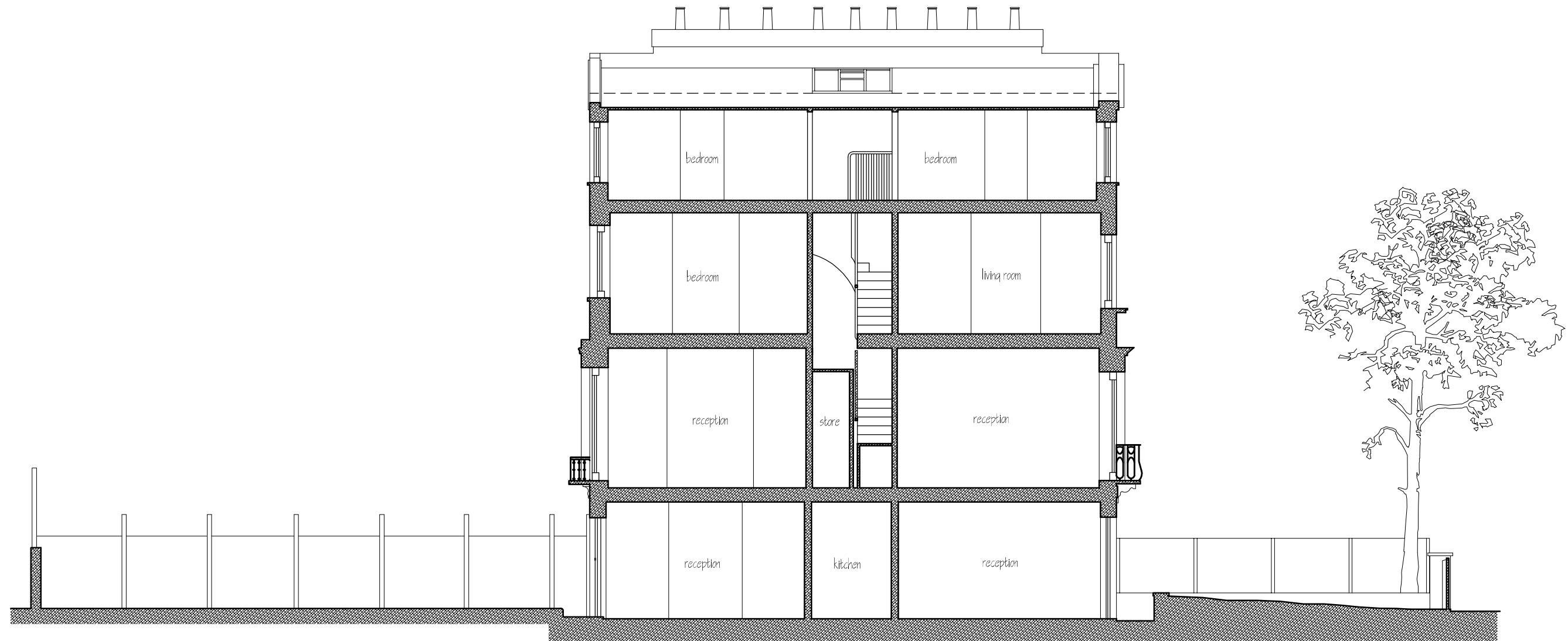
LONGITUDINAL SECTION A-A - (AS EXISTING)
