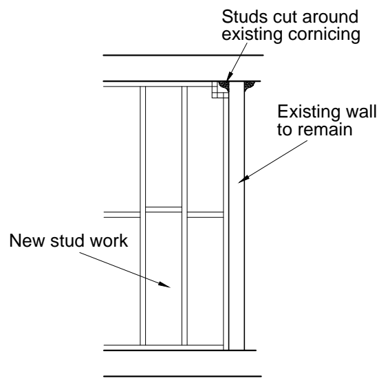
DETAIL B scale 1:50
