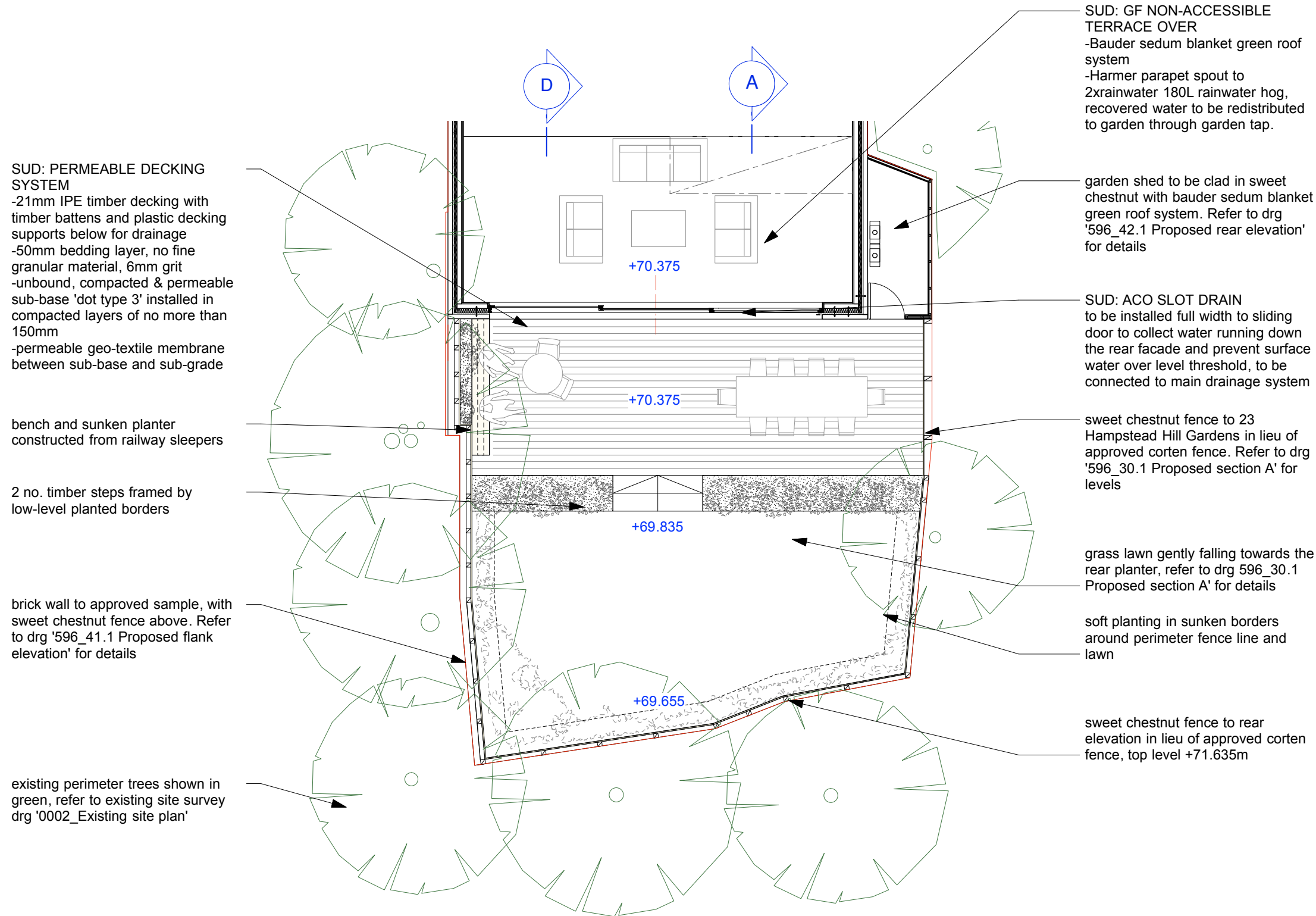
1 Proposed rear landscape plan Scale: 1:100
