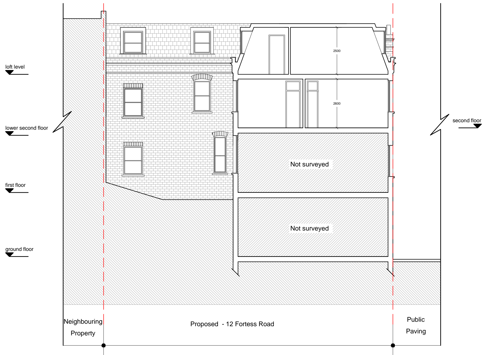
SECTION CC'
