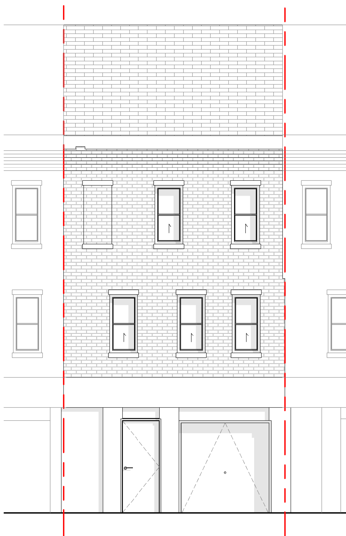
1 Front Elevation - Existing 1 : 50
