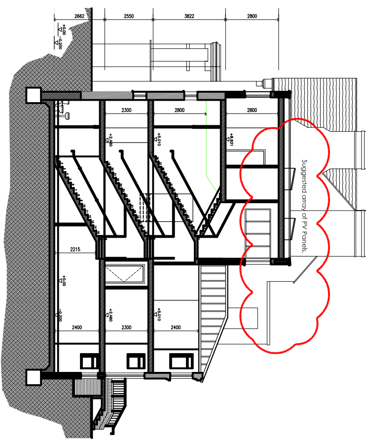
proposed section through B-B
