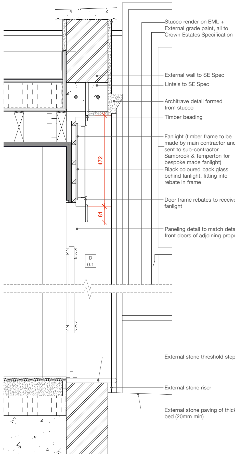
D2 Section detail of front door Scale 1:10
