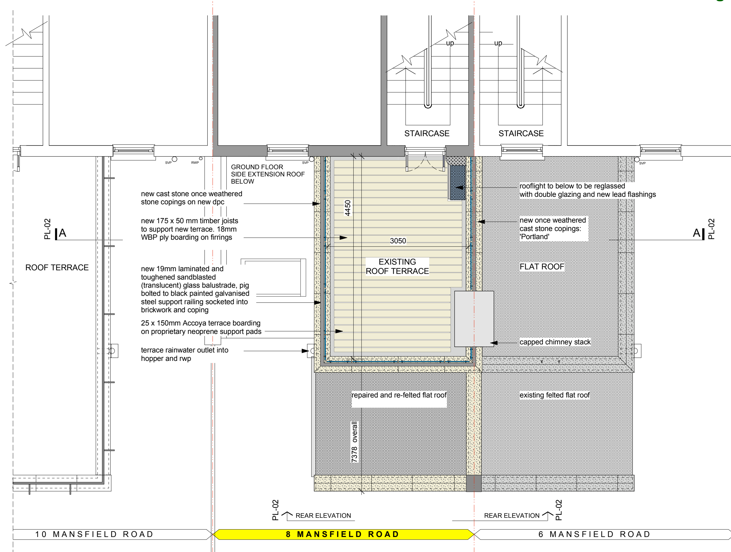
PROPOSED PLAN OF NEW RAILINGS AND GLASS SCREEN TO EXISTING REAR ROOF TERRACE 1-50
