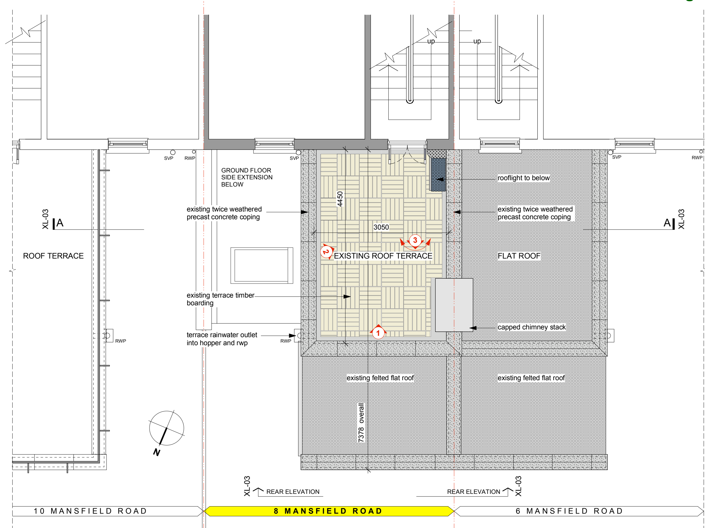
EXISTING REAR EXTENSION ROOF TERRACE PLAN 1-50
