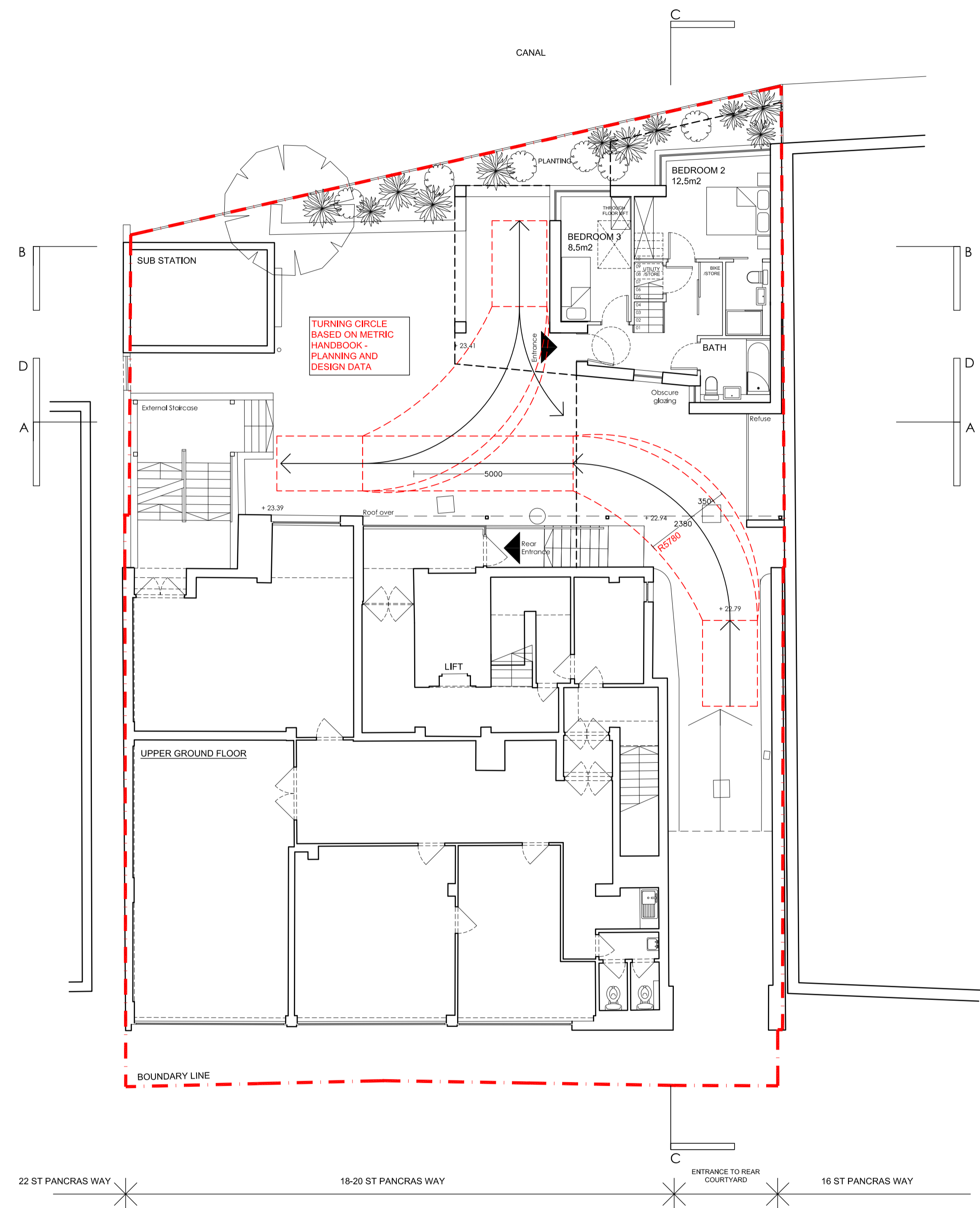
UPPER GROUND FLOOR
