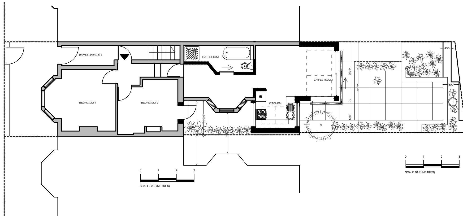
05 PROPOSED GROUND FLOOR PLAN A-(13)-010 1:50 @ A1, 1:100 @ A3
