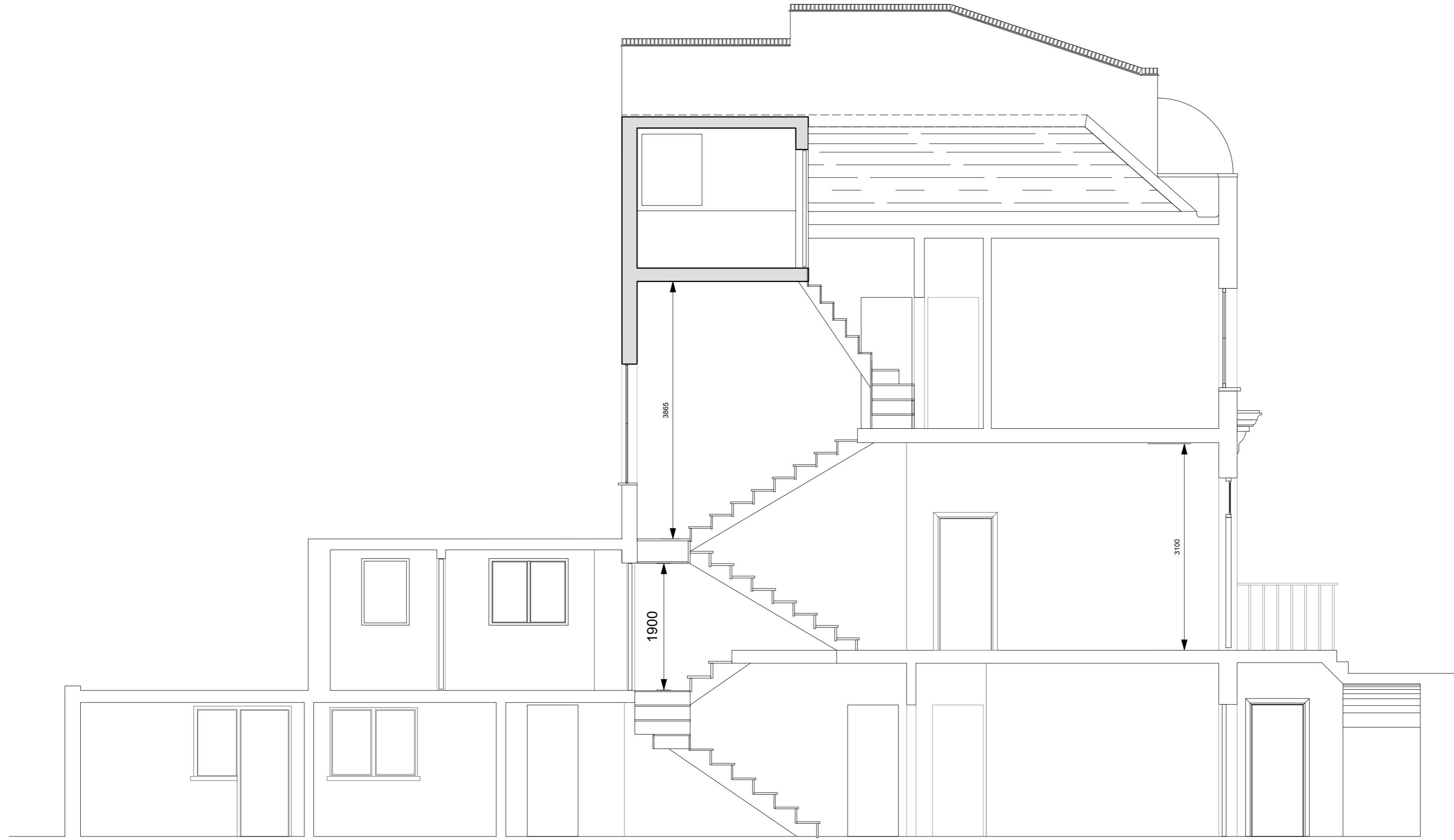
Section AA
