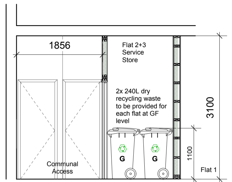
Section CC
