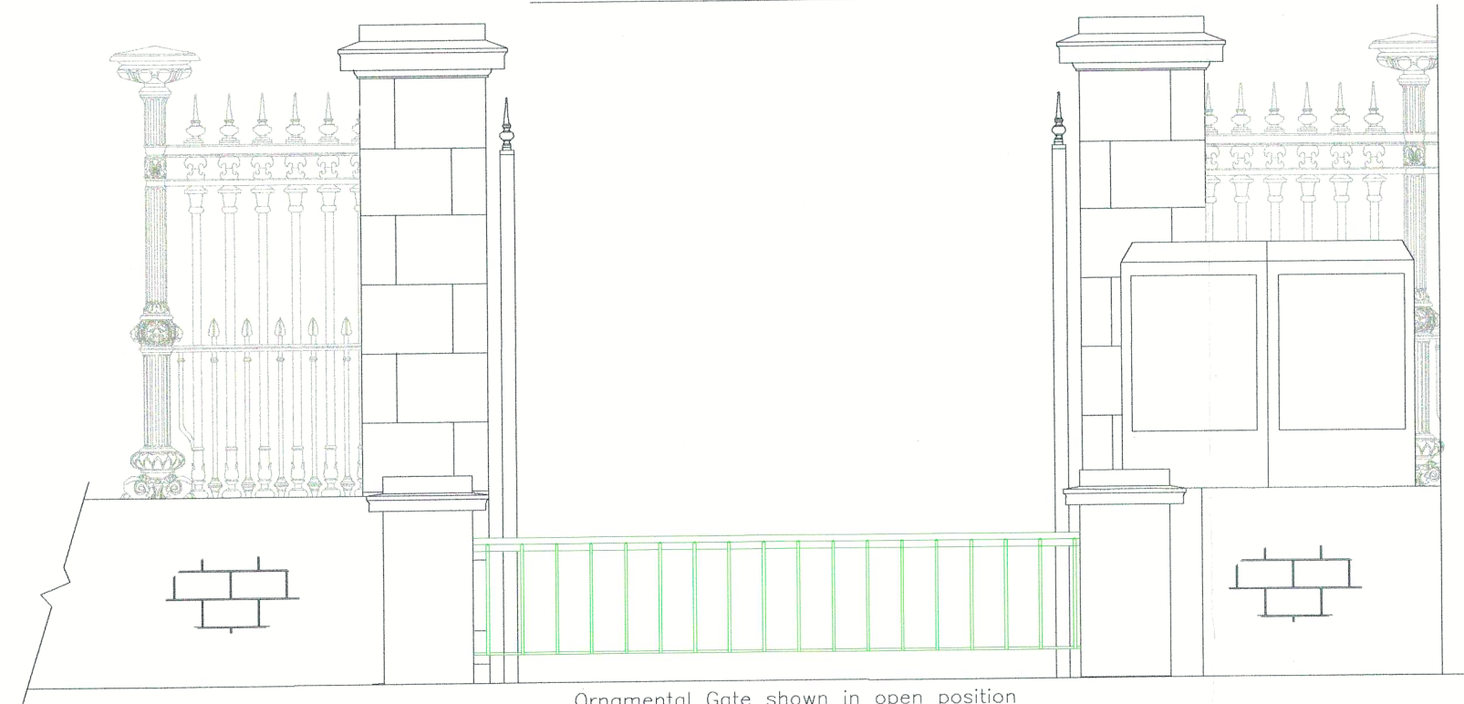
Ornamental Gate shown in open position ELEVATION TOWARDS STREET
