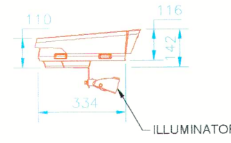
STATIC BODY CAMERA 5M ILLUMINATOR
