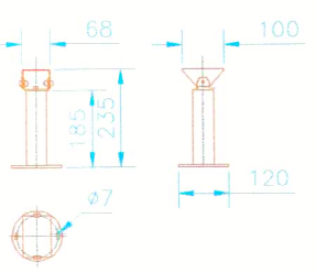
COLUMN MOUNT BALL JOINT DETAILS
