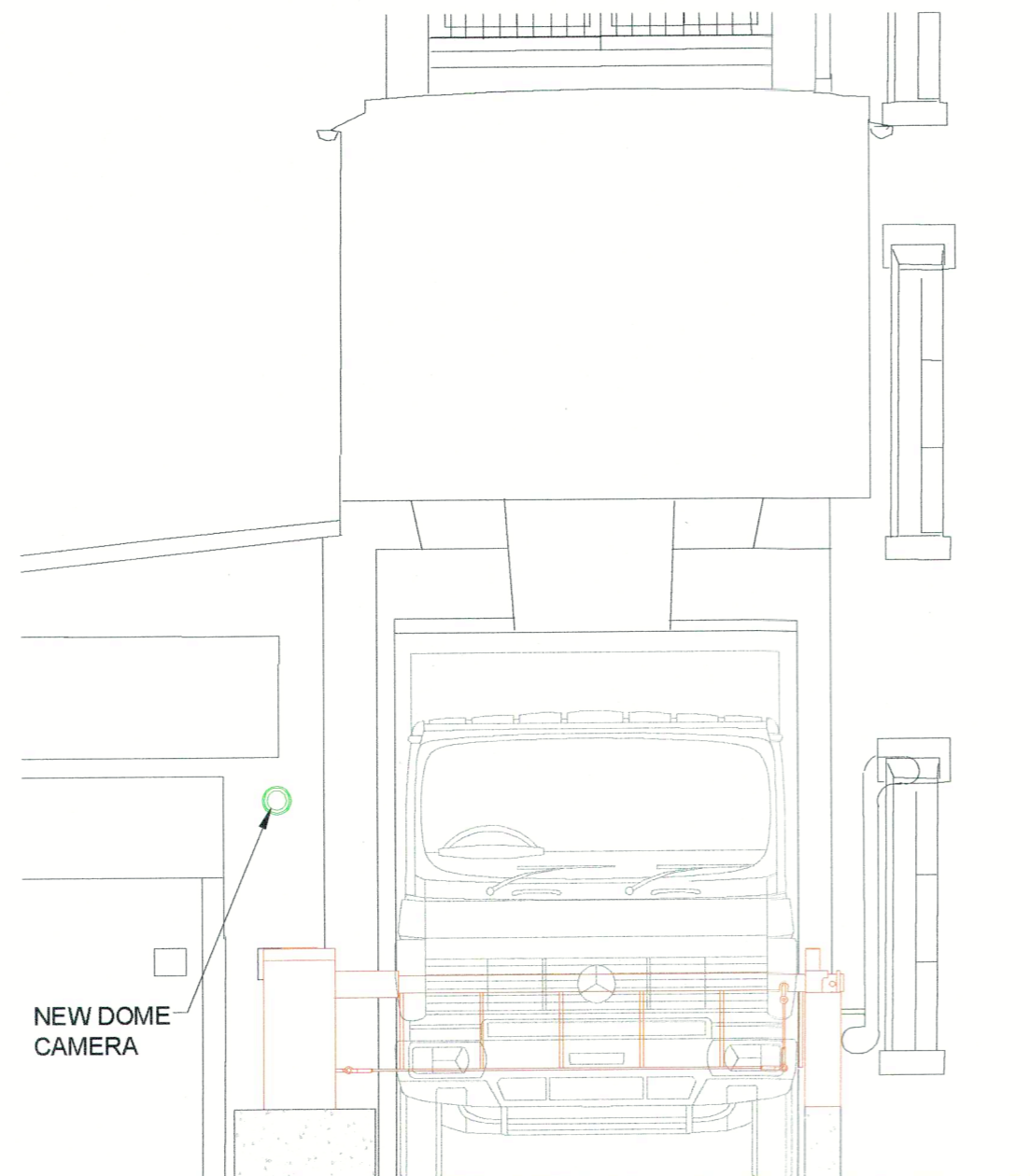
REAR ELEVATION (TOWARDS MONTAGUE PLACE) VEHICLE ENTERING SITE (Scale 1:50)
