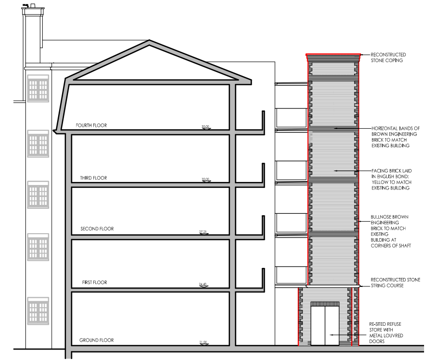
PROPOSED NEW SIDE ELEVATION TO NORTH
