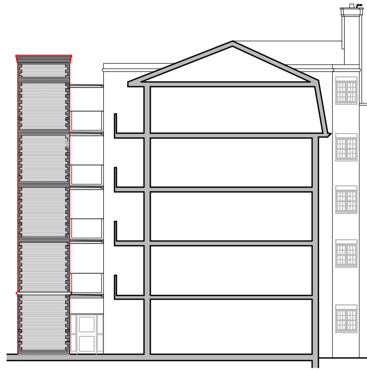
PROPOSED NEW SIDE ELEVATION TO SOUTH
