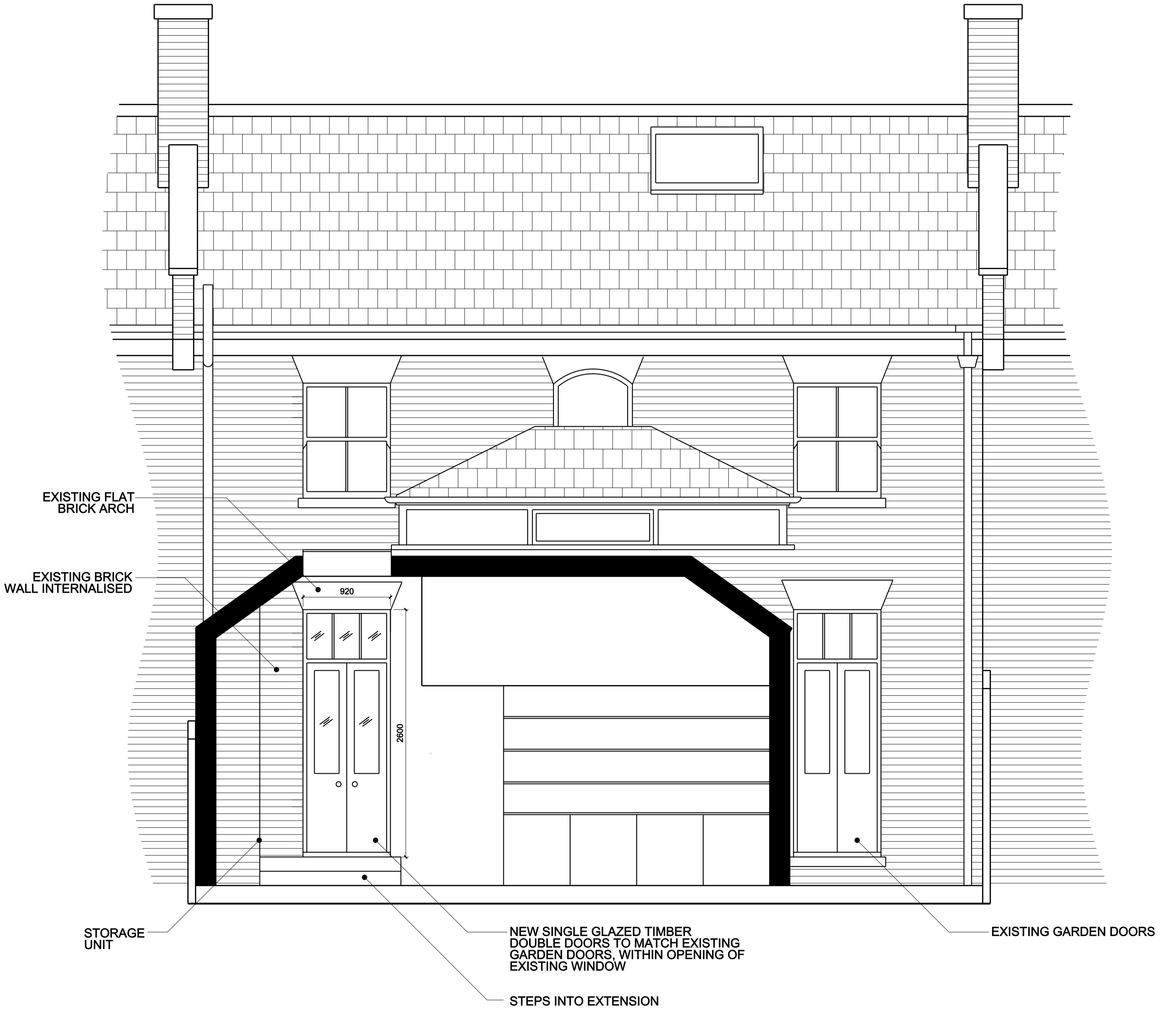
1 1:25 LIVING ROOM INTERNAL ELEVATION
