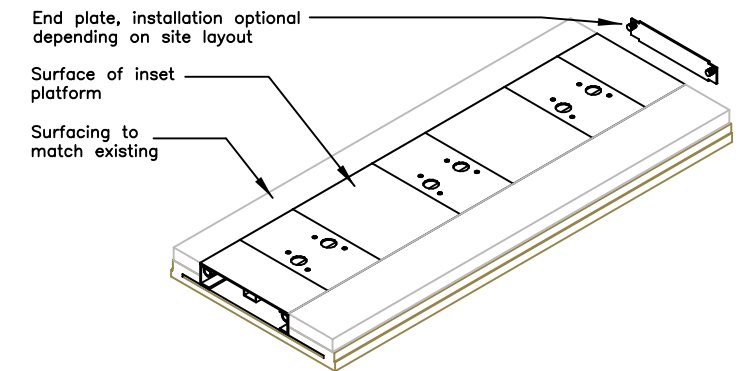
ISOMETRIC DIAGRAM (FOR ILLUSTRATIVE PURPOSES ONLY)
