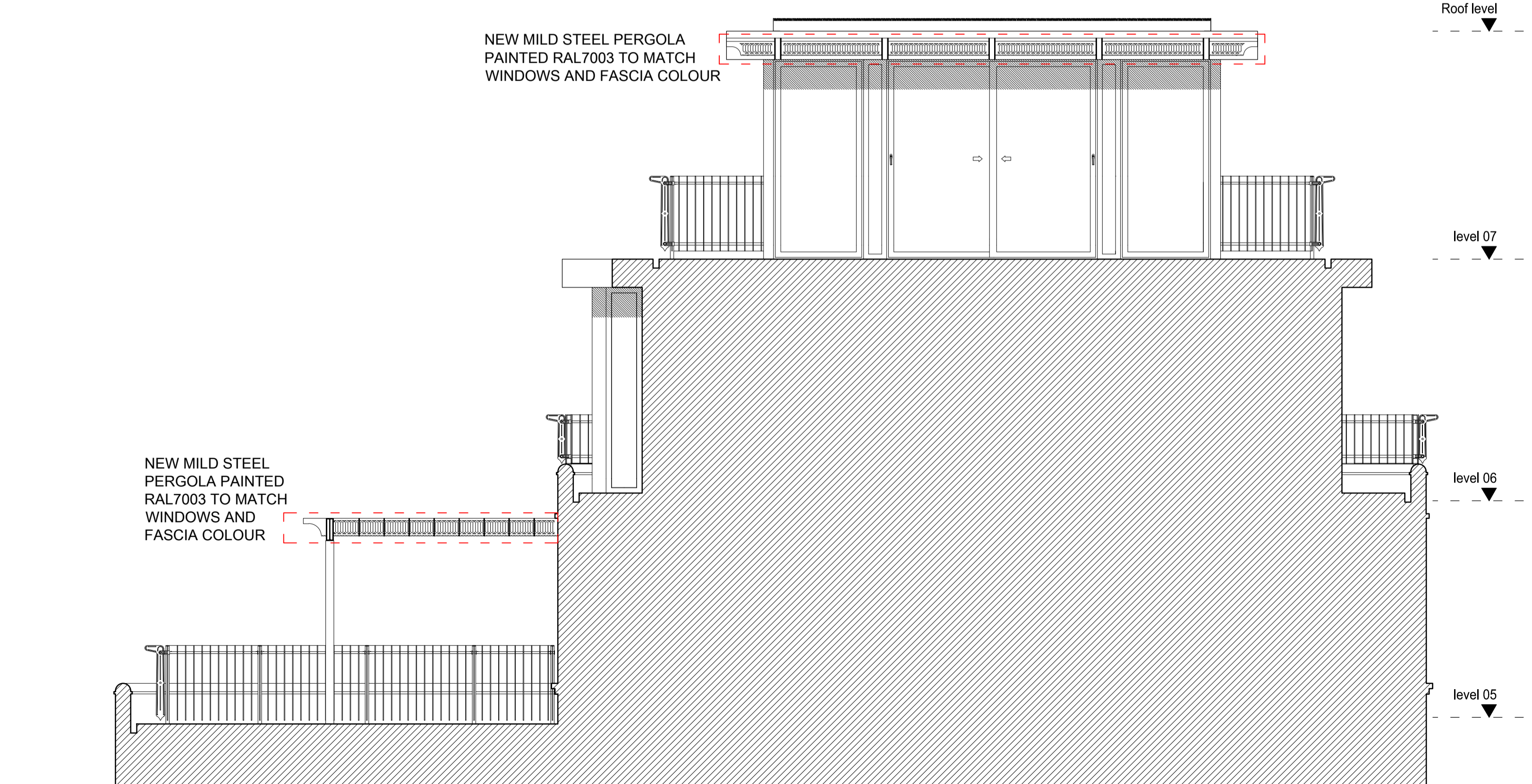
PROPOSED SECTION C-C'
