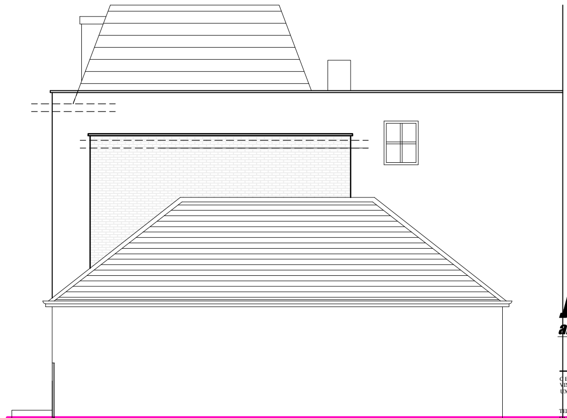
SOUTH-EAST ELEVATION
