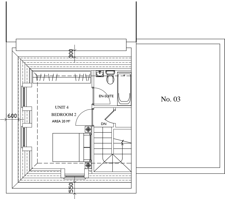
PROPOSED MANSARD ROOF PLAN
