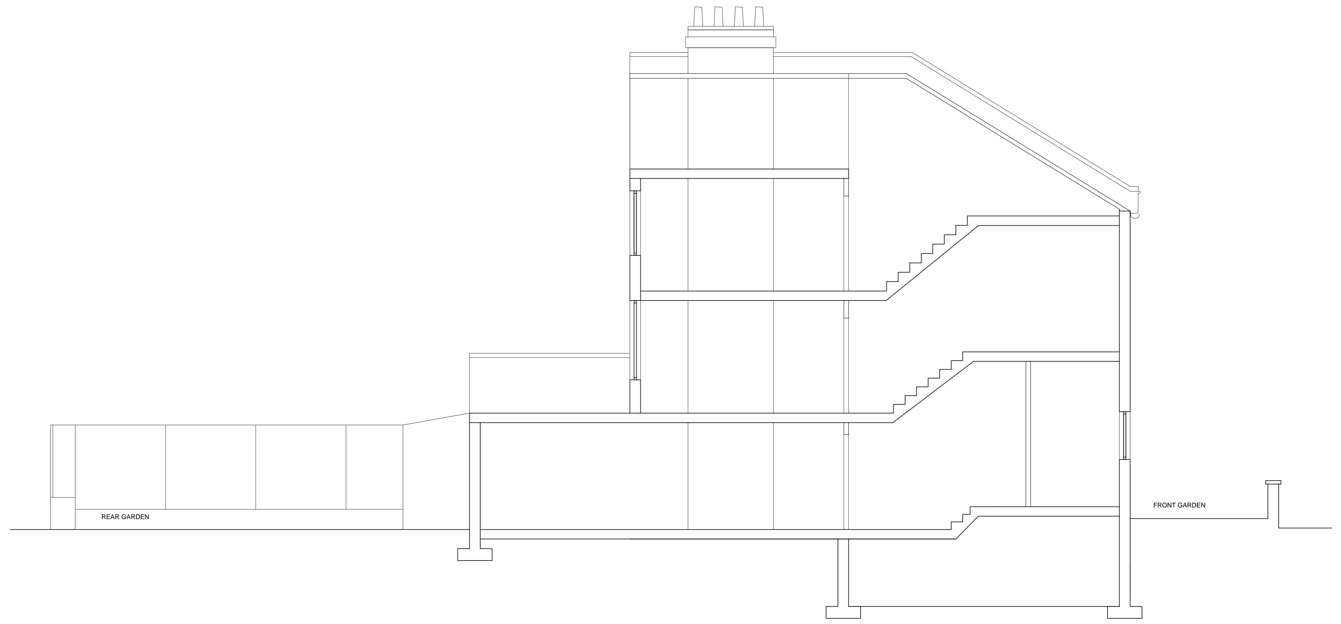
EXISTING SECTION B-B
