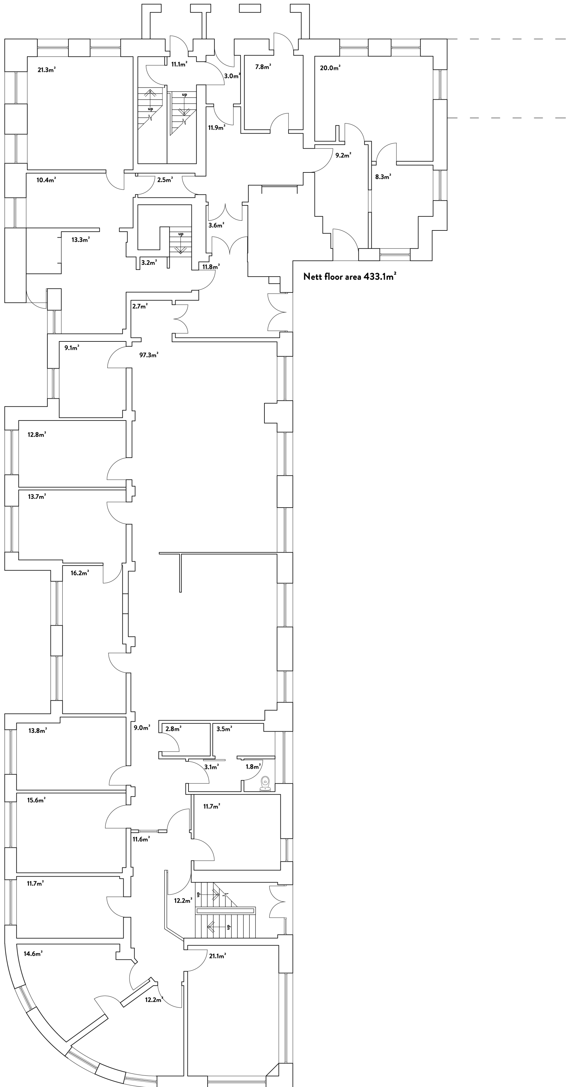
TH00 Proposed Ground Floor Plan National Temperance Hospital Insull Wing Hampstead Road London
