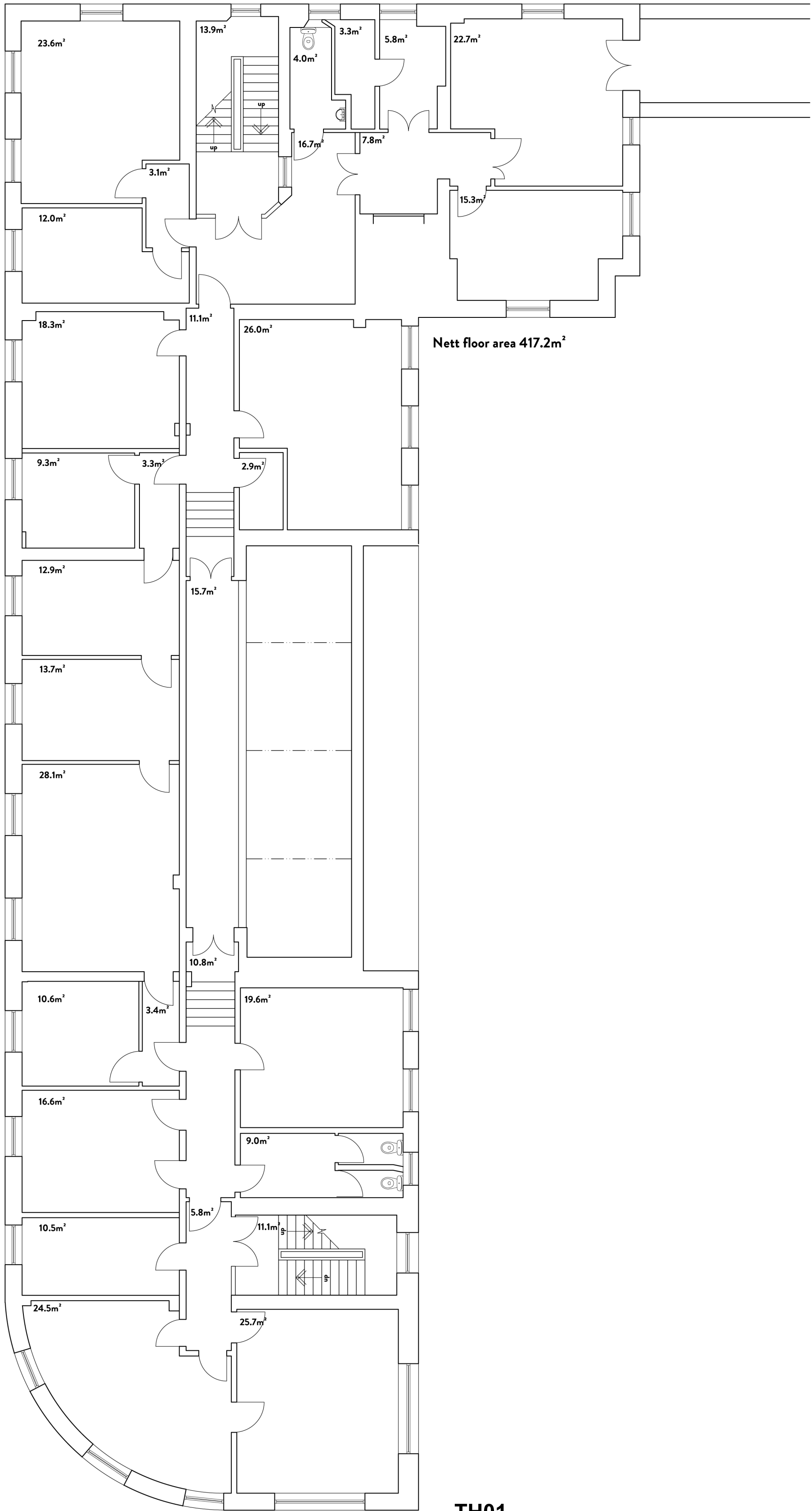
TH01 Proposed First Floor Plan National Temperance Hospital Insull Wing Hampstead Road London
